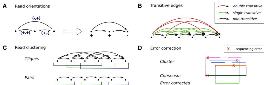
Figure 5. Algorithmic details. (A) Read orientations: Given an edge u \rightarrow v with orientations (-,+) . Then, if u is labeled +, the induced label for v is −, while if u is labeled −, the induced label for v is +. This procedure leads to a vertex labeling in O(V) time. (B) Transitive edges: An edge u \rightarrow w is called nontransitive , shown in black, if there is no vertex v such that there are edges u \rightarrow v , v \rightarrow w . It is called single transitive , shown in green, if for all vertices v such that there are edges u \rightarrow v , v \rightarrow w , one of the edges is nontransitive. It is called double transitive , shown in red, if there is a vertex v with edges u \rightarrow v , v \rightarrow w which are both transitive. (C) Read clustering by cliques ( top ) or by pairs ( bottom ). (D) Error correction: When a consensus sequence is constructed from a cluster of reads, the extremities are removed.
