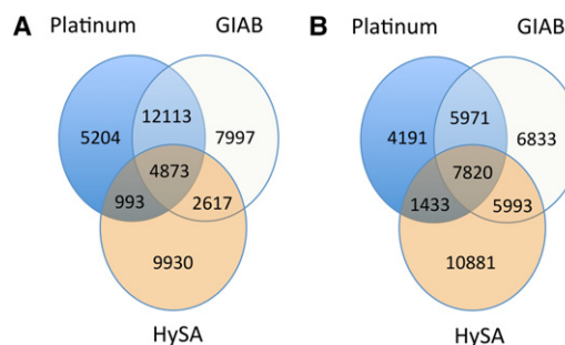
Figure 3. Comparison of small indels detected in NA12878 by HySA with those in the Platinum and GIAB sets. (A) Deletions with 1-bp overlap criterion. (B) Insertions with 1-bp overlap criterion allowing 50-bp offset on the left and right of the insertion breakpoints.
