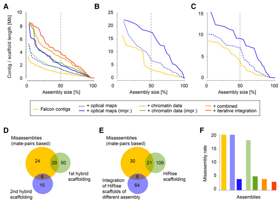
Figure 1. Assembly results and strategies. (A–C) Assembly contiguity of the assemblies of three species: A. alpina (A), E. syriacum (B), C. planisiliqua (C). The x-axis indicates the cumulative length of contigs sorted by length (expressed as percent of the entire assembly). The y-axis shows individual contig or scaffold length. The dashed line indicates the N50/L50 values. (D) Misassemblies identified with Illumina mate-pairs (yellow) and their overlap with breaks introduced during misassembly identification using optical maps (in two steps shown in green and blue). (E) Misassemblies identified with Illumina mate-pair alignments (yellow) and their overlap with breaks introduced during our integration of Dovetail Genomics chromosome conformation capture data (again, two steps shown in green and blue). (F) Inter-chromosome misassemblies identified by a genetic map in each of the assemblies (as shown in A).
