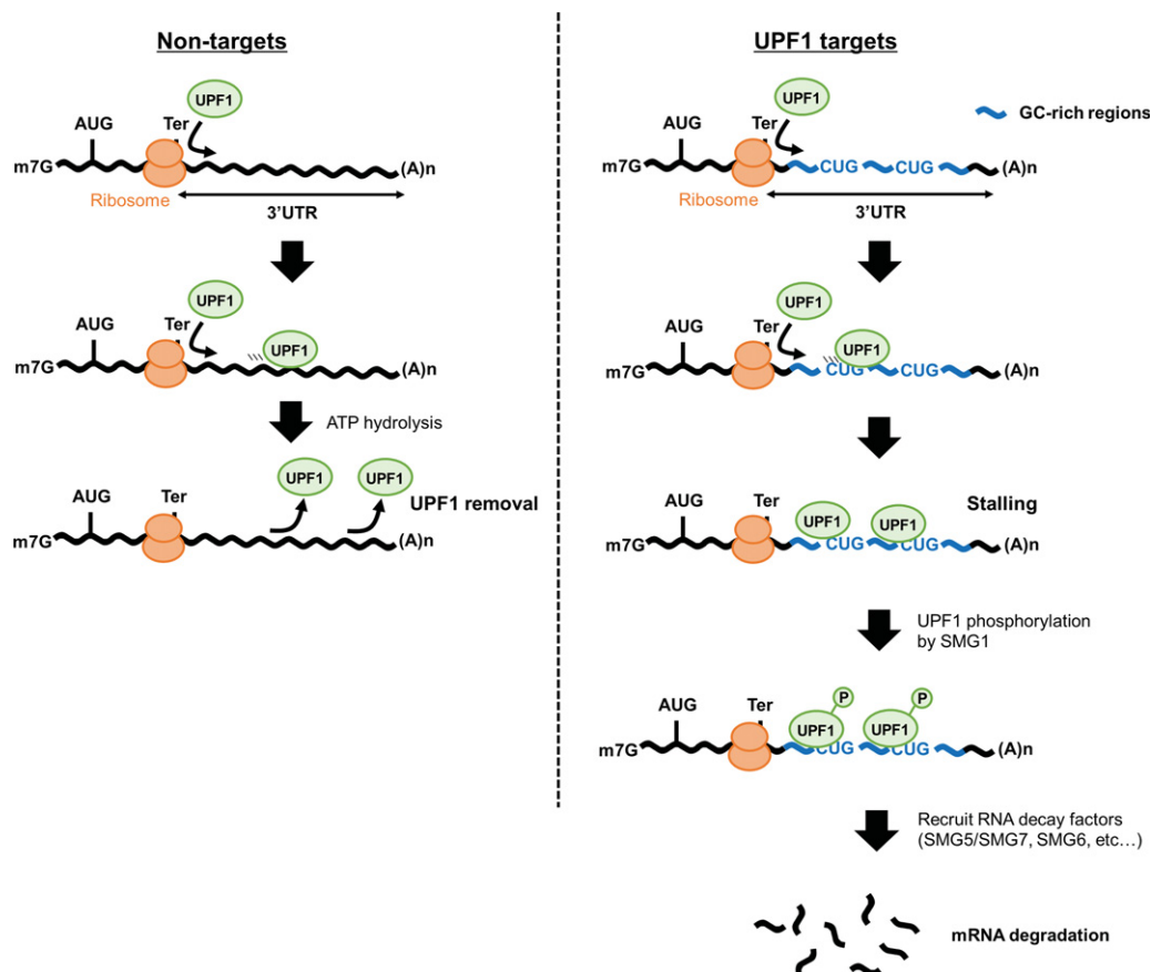
Figure 6. Model for the mechanism of UPF1-dependent mRNA decay. UPF1 protein is loaded onto target mRNAs via translation and then translocates over the 3' UTR. In non-GC-rich regions ( left ), UPF1 is removed from mRNAs. In contrast, in GC-rich regions ( right ), UPF1 stalls at CUG-centered GC-rich motifs, which promotes mRNA decay.
