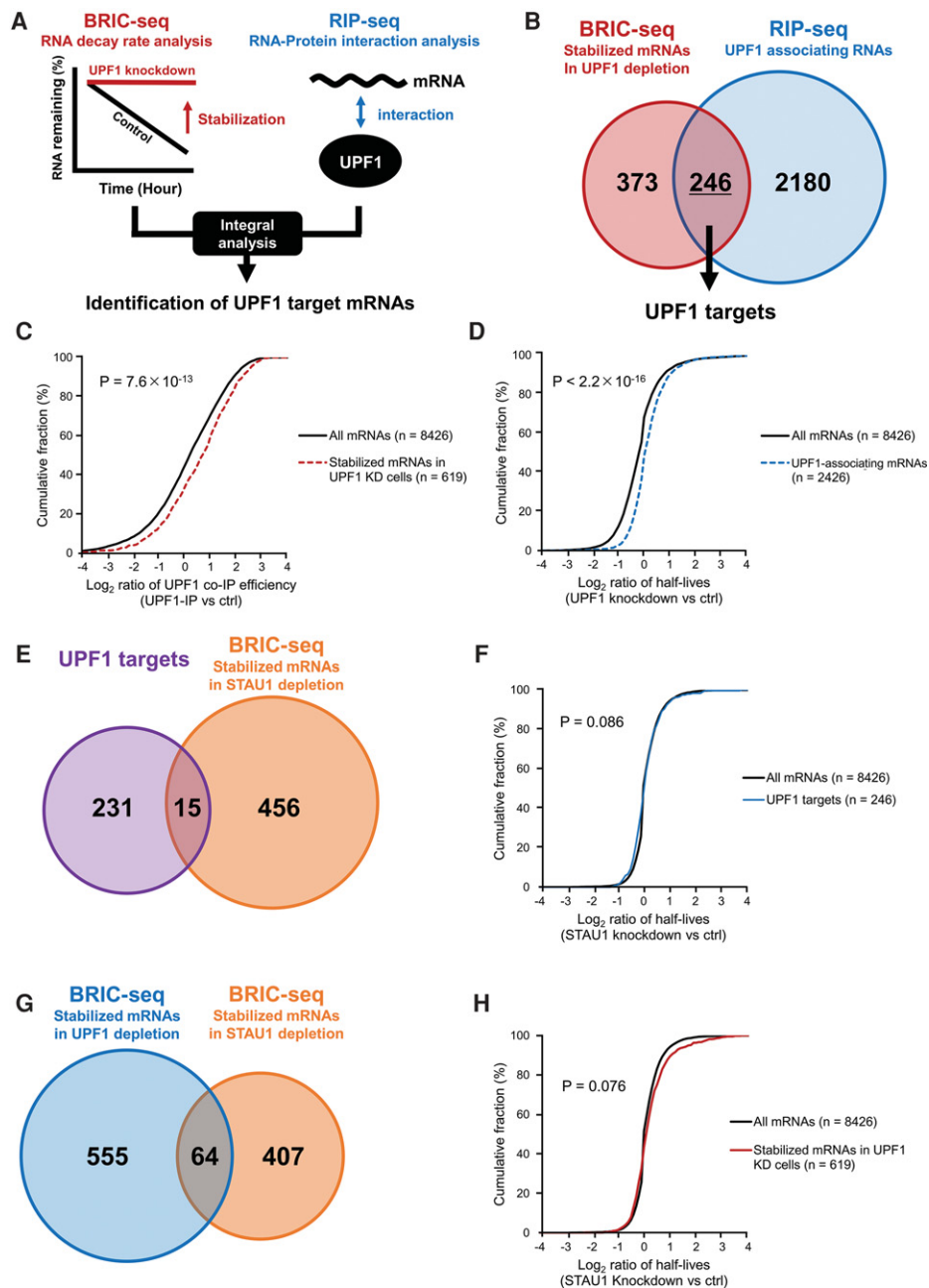
Figure 1. Identification of UPF1 and SMD target mRNAs, including UPF1 targets partially regulated by the STA1 protein. (A) Schematic of the method to identify UPF1 targets based on the combinatorial analysis of BRIC-seq and RIP-seq. (B) Venn diagram illustrating the overlap of the two types of mRNAs: those with more than twofold prolonged half-lives upon UPF1 -knockdown in HeLa tet-off cells (red: BRIC-seq, 619 mRNAs) and those enriched by more than twofold in the HA-UPF1 immunoprecipitation fraction relative to input fraction (blue: RIP-seq, 2426 mRNAs). The intersection of stabilized mRNAs in UPF1 -knockdown cells (BRIC-seq) and UPF1-associating mRNAs (RIP-seq) were judged as bona fide UPF1 target mRNAs (246 mRNAs). (C) Cumulative distribution of changes in UPF1 association of 619 transcripts stabilized upon UPF1 depletion (red dashed line; median: 0.66) and 8426 whole transcripts (black solid line; median: 0.17). Changes in UPF1 association were calculated as the number of mapped tags of RNA-seq immunoprecipitated with HA-UPF1 by reads per kilobase of transcript per million mapped reads [RPKM]/the number of mapped tags of input RNA-seq [RPKM] \geq 2 . P -values were calculated using the Wilcoxon rank-sum test. (D) Cumulative distribution of changes in RNA stability of 2426 UPF1 associating transcripts (blue dashed line; median: 0.02) and 8426 whole transcripts (black solid line; median: -0.20 ). Changes in RNA stability were determined by the following calculation: the half-life of each transcript in UPF1 depletion/the half-life of each transcript in control. P -values were calculated using the Wilcoxon rank-sum test. (E) Venn diagram illustrating the overlap of two types of genes: UPF1 target mRNAs (purple: 246 genes) and mRNAs with more than twofold prolonged half-lives upon STA1 -knockdown in HeLa tet-off cells (orange: BRIC-seq, 471 genes). The intersection of the UPF1 target mRNAs and stabilized mRNAs in STA1 -knockdown cells (BRIC-seq) indicates STA1-mediated mRNA decay (SMD) target mRNAs (15 genes). (F) Cumulative distribution of changes in RNA stability of 246 UPF1 target transcripts (blue line; median: 0.032) and 8426 whole transcripts (black line; median: 0.000). Changes in RNA stability were determined by the following calculation: the half-life of each transcript in STA1 depletion/the half-life of each transcript in control. P -values were calculated using the Wilcoxon rank-sum test. (G) Venn diagram illustrating the overlap of two types of mRNAs: those with more than twofold prolonged half-lives upon UPF1 -knockdown (blue: BRIC-seq, 619 genes containing 246 UPF1 targets and 373 transcripts stabilized by UPF1 depletion but not associated with UPF1; see B) and STA1 -knockdown in HeLa tet-off cells (orange: BRIC-seq, 471 genes). The number of the stabilized mRNAs upon UPF1 -knockdown (BRIC-seq) and those upon STA1 -knockdown (BRIC-seq) contains 64 mRNAs. (H) Cumulative distribution of changes in RNA stability of mRNAs with more than twofold prolonged half-lives upon UPF1 -knockdown (red line; median: 0.008) and 8426 whole transcripts (black line; median: 0.000). Changes in RNA stability were determined by the following calculation: the half-life of each transcript in STA1 depletion/the half-life of each transcript in control. P -values were calculated using the Wilcoxon rank-sum test.
