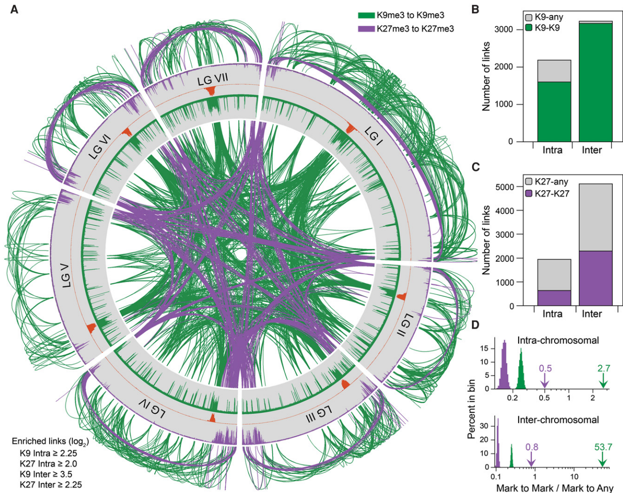
Figure 2. Predicted networks of H3K9me 3 -marked and H3K27me 2/3 -marked regions. (A) Plot of frequently observed contacts between heterochromatic regions from all seven chromosomes (LGI–LGVII) at 10-kb resolution. Green and purple links indicate frequent contacts between regions enriched with H3K9me 3 or H3K27me 2/3 , respectively. Links inside and outside the plot show inter- and intra-chromosomal associations, respectively. The near absence of subtelomeric interactions between H3K27me 2/3 -enriched regions on LGV may reflect the incomplete assembly of the rDNA repeats on the LGV left arm. (B) Summary of observed levels of strong intra- and inter-chromosomal links between regions enriched with H3K9me 3 (green bars) or between H3K9me 3 -enriched regions and regions without H3K9me 3 (gray bars), generated with the script matrix2CircosK9Quant.py . (C) Summary of strong intra- and inter-chromosomal links between regions enriched with H3K27me 2/3 (purple bars) or between regions enriched with H3K27me 2/3 and regions without H3K27me 2/3 (gray bars), generated with the script matrix2CircosK27Quant.py . (D) Distributions of ratios of interactions of like (Mark to Mark) or unlike (Mark to Any) regions from 10,000 randomly generated arrangements of strong intra- and inter-chromosomal contacts originating from H3K9me 3 -enriched regions (green) or H3K27me 2/3 -enriched regions (purple), produced by the scripts K9RandomizeInter.py , K9RandomizeIntra.py , K27RandomInter.py , and K27RandomizeIntra.py . The observed ratios of specific to nonspecific contacts for the H3K9me 3 and H3K27me 2/3 networks are denoted with green and purple arrows, respectively, and correspond to the plots in B and C.
