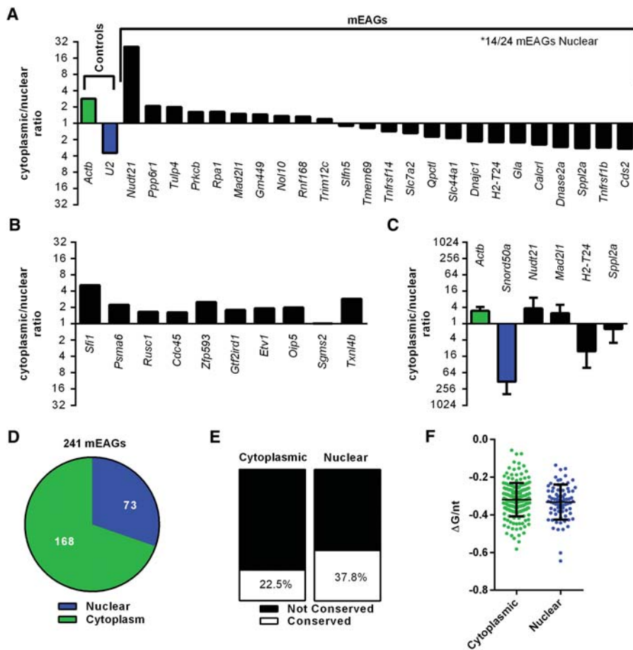
Figure 5. A subset of mEAG transcripts is enriched in the nucleus. Data sets for unstimulated BMDMs (Bhatt et al. 2012) were used to determine the cytoplasmic to nuclear ratio of transcripts for (A) controls and TOP25 mEAGs and (B) 10 randomly selected protein-coding genes. (C) Validation of controls and mEAGs using qRT-PCR of RNA isolated from nuclear or cytoplasmic fractions of unstimulated RAW264.7 macrophages. (D) Predominant cellular localization for all mEAGs using Bhatt et al. data sets. (E) Predominant cellular localization of EAGs found in orthologs of both mouse and human. P=0.01242 by Z test for two population proportions. (F) Folding free energy per nucleotide ( \Delta G/nt ) for cytoplasmic and nuclear-localized mEERs. P=0.9109 using Mann-Whitney U test.
