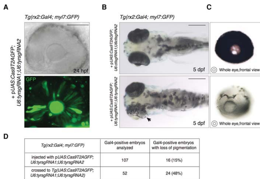
Figure 2. Tissue-specific disruption of the tyrosinase locus induced by the expression of the UAS-based vector in the retinal progenitor cells. (A) Transmitted light and confocal imaging of eye of a 24 hpf Tg(rx2:Gal4;myl7:GFP) embryo injected with pUAS: Cas9T2AGFP ; U6:tyrsgRNA1 ; U6:tyrsgRNA2 together with Tol2 mRNA. GFP fluorescence indicates Gal4 -driven expression of the Cas9 enzyme in the retinal progenitor cells (RPCs) giving rise to the retinal pigmented epithelium (RPE) and to the neural retina. Scale bar = 100 \mu m. (B) (Lower panel) Specific loss of pigmentation in the RPE of a 5 dpf zebrafish embryo induced by injection of pUAS: Cas9T2AGFP ; U6:tyrsgRNA1 ; U6:tyrsgRNA2 in Tg(rx2:Gal4; myl7:GFP) at one-cell stage. Arrowhead indicates the eye with lost pigmentation. (Upper panel) Control embryo injected with the same vector containing a control sgRNA sequence ( ctfsgRNA ). Scale bar = 300 \mu m. (C) Frontal view of eyes with absent pigmentation (lower panel) and wild-type (upper panel) explanted from the larvae shown in B. (D) Table showing the percentage of Gal4 -positive larvae displaying loss of pigmentation in the RPE. (First row) Injection of the pUAS: Cas9T2AGFP ; U6:tyrsgRNA1 ; U6:tyrsgRNA2 into one-cell-stage Tg(rx2:Gal4; myl7:GFP) embryos. (Second row) Cross of Tg(rx2:Gal4; myl7:GFP) fish with Tg(UAS:Cas9T2AGFP;U6:tyrsgRNA1;U6:tyrsgRNA2) .
