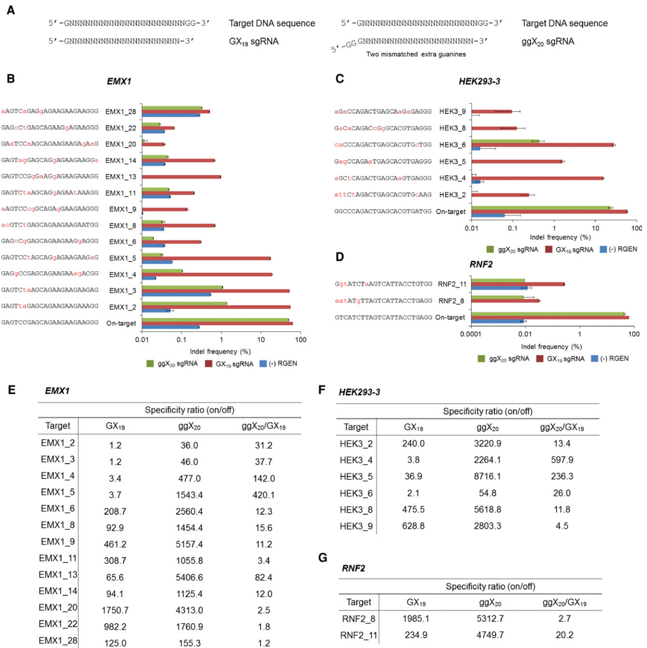
Figure 4. Indel frequencies determined using targeted deep sequencing at off-target sites. (A) Schematic of conventional sgRNAs (GX 19 sgRNA) and modified sgRNAs (ggX 20 sgRNA). Indel frequencies at NGS-validated on- and off-target sites for the EMX1 (B), HEK293-3 (C), and RNF2 sgRNAs (D). Specificity ratios calculated by dividing the indel frequency at the on-target site with that at an off-target site for the EMX1 (E), HEK293-3 (F), and RNF2 sgRNAs (G).
