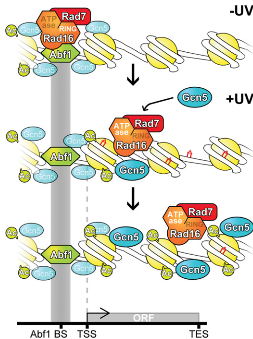
Figure 9. Model to illustrate how GG-NER is organized in the yeast genome. (Top panel) In undamaged cells, the GG-NER complex is located at multiple Abf1 binding sites predominantly in the promoter regions of genes. This occupancy is dependent on the RING domain of the Rad16 protein. The enrichment of GG-NER-independent basal levels of Gcn5 can be detected at these sites. (Middle panel) In response to UV irradiation, the GG-NER complex dissociates from the Abf1 component at Abf1 binding sites. This process depends on the activity of the ATPase domain in Rad16. Concomitantly, the HAT Gcn5 is recruited onto the chromatin with its increased levels and distribution dependent on the Rad7-Rad16 GG-NER complex. (Bottom panel) During this process, histone H3 acetylation is increased over a domain defined by the redistribution of the Rad7-Rad16 proteins from Abf1 binding sites. This mechanism drives the chromatin remodeling necessary for the efficient repair of UV damage.
