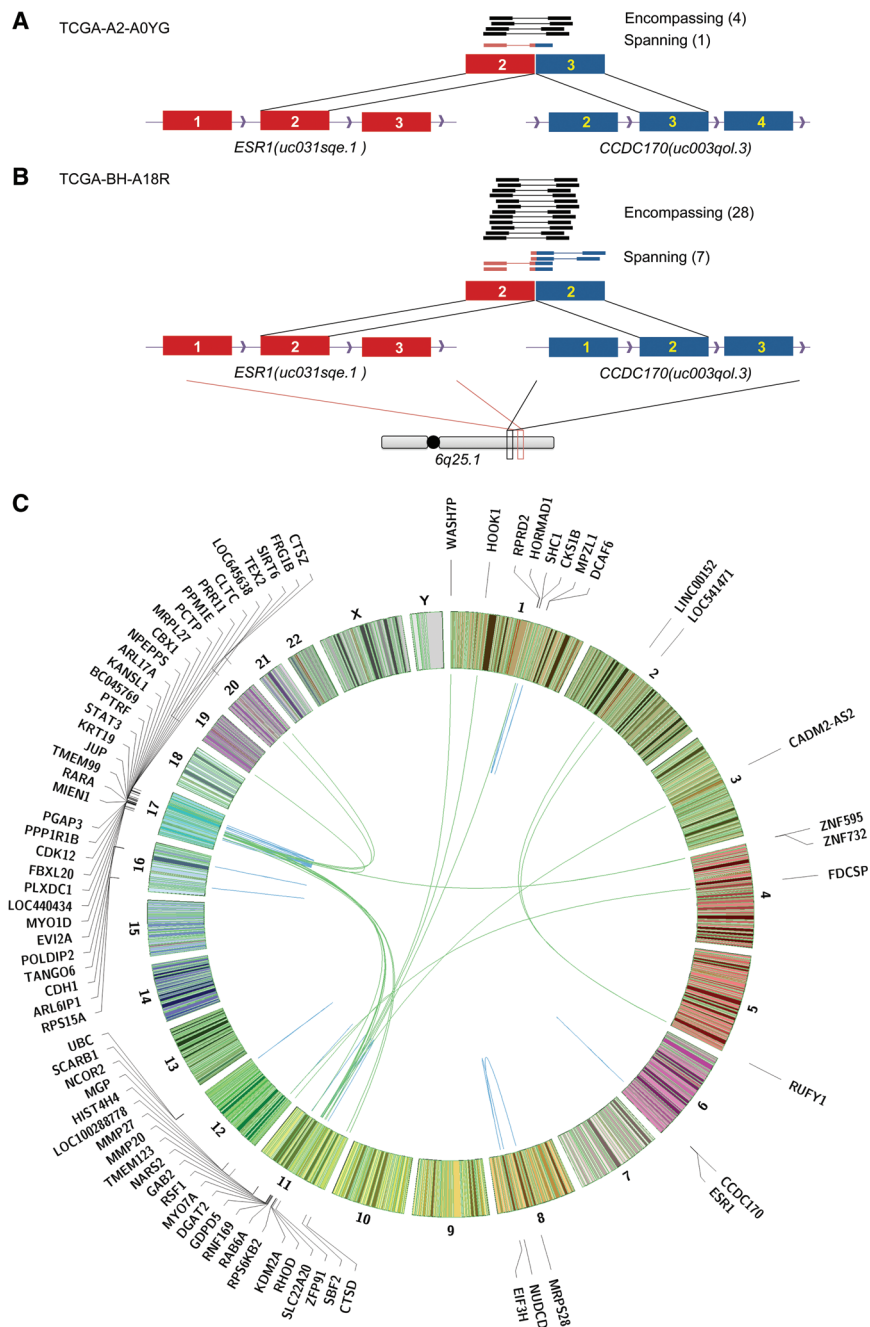
Figure 5. Hotspots of gene fusions in 62 TCGA breast cancer patients. (A) ESR1 - CCDC170 fusion in TCGA-A2-A0YG. (B) ESR1 - CCDC170 fusion in TCGA-BH-A18R. ESR1 (red) and CCDC170 (blue) are on the forward strand in region 6q25.1, and the 5' gene ESR1 is downstream from the 3' gene CCDC170 . The two fusions share the same 5' exon at ESR1 (Exon 2 of transcript uc031sqe.1), but 3' exons of CCDC170 are different (Exons 2 and 3 of transcript uc003qol.3). (C) Circos plot of recurrent and functionally recurrent gene fusions detected by INTEGRATE. The green lines indicate inter-chromosomal gene fusions, and the blue lines indicate intra-chromosomal gene fusions. The names of the genes involved in each fusion are plotted on the outside of the circle. The gene fusions associate with several hotspots on Chromosomes 1, 11, and 17.
