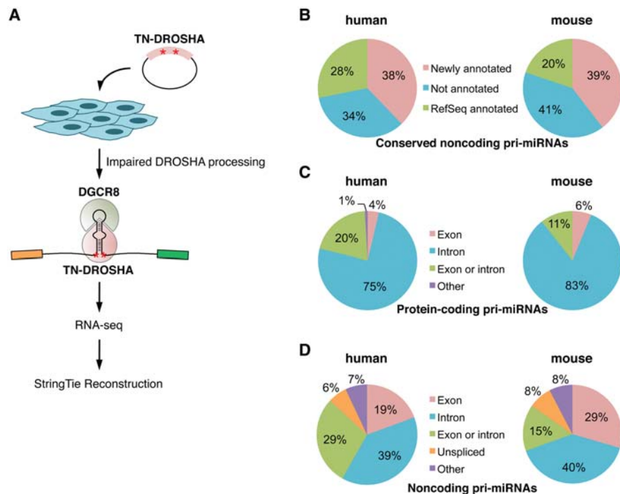
Figure 2. General characteristics of human and mouse pri-miRNAs. (A) Overview of the experimental workflow used to generate pri-miRNA assemblies. (B) Proportion of conserved non-protein-coding human and mouse pri-miRNAs annotated in this study or in RefSeq in at least one cell type. (C,D) Intronic or exonic locations of conserved miRNAs transcribed within protein-coding (C) or non-protein-coding genes (D).
