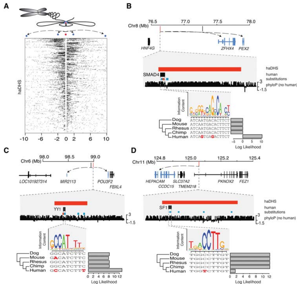
Figure 6. Hi-C chromatin conformation data identify putative regulatory targets of haDHSs. (A) Contacts are shown for all haDHSs, and each row indicates the contacts for one haDHS, which is in the center . Black boxes indicate one 40-kb contact region. The schematic above illustrates how chromatin conformation information gets translated into the Hi-C contact data. Blue dots represent contact regions; the red dot, an haDHS. (B–D) Three example haDHSs are shown with their surrounding genes and a predicted transcription factor binding site that is affected by a human-specific mutation(s). Genes that contact the haDHSs in Hi-C data are highlighted in blue, with arrows pointing to their transcription start sites. Examples B and C depict substitutions that create transcription factor binding sites, while D is a binding site that is predicted to be lost in humans. Human-specific substitutions that go from a weak to a strong base are shown in red, while all other substitutions are shown in blue. Bar plots, FIMO (Grant et al. 2011) log likelihood ratios of motif calls in each species.
