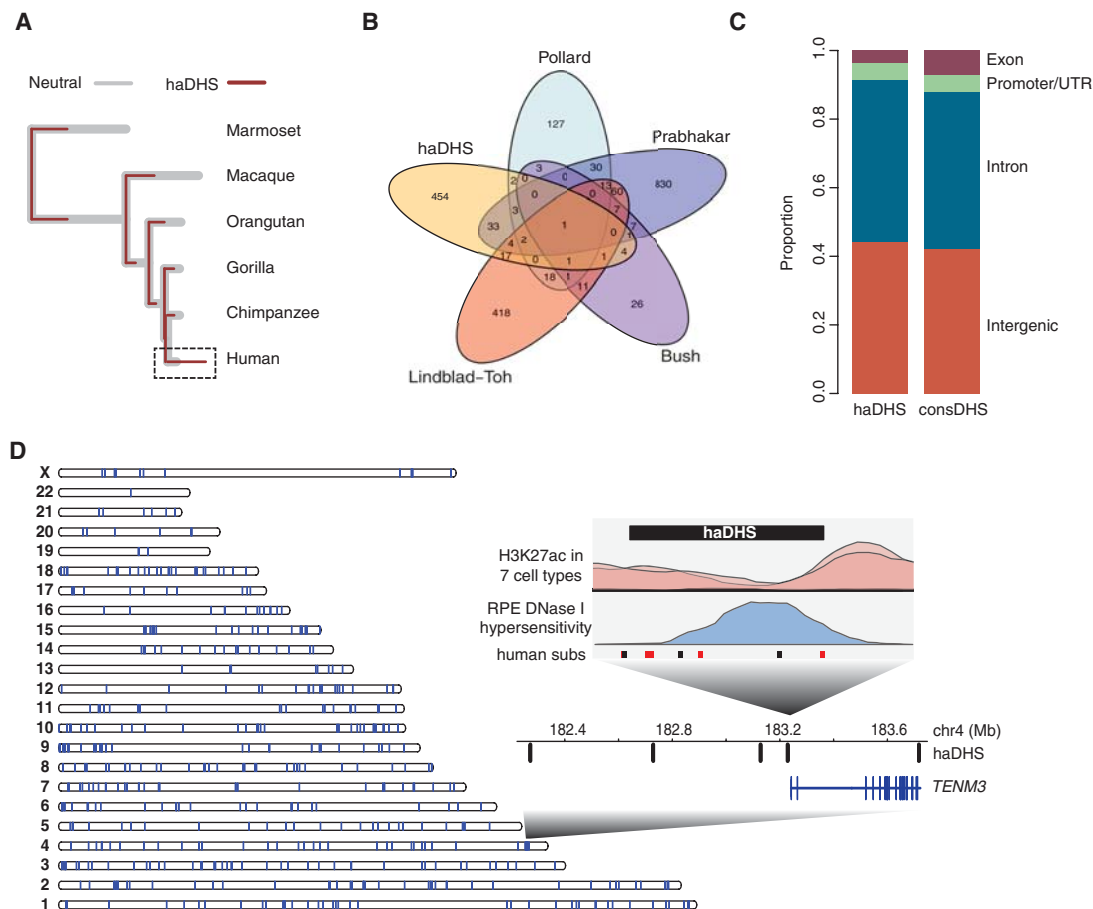
Figure 3. Characteristics of human-accelerated DHSs. (A) Overlaid phylogenetic trees inferred in haDHSs (maroon) versus their flanking neutral regions (gray). The human branch is highlighted by the dashed rectangle. (B) Venn diagram showing overlap of haDHSs with human accelerated elements (HAEs) identified in previous studies. (C) The proportion of bases in haDHSs and conserved DHSs that are located in different functional classes of genomic sequence. (D) Distribution of haDHSs across the genome. Each vertical bar on the chromosome ideogram represents an haDHS. (Inset) Plot shows a region on Chromosome 4 near the TENM3 gene that contains five haDHSs. The fourth haDHS is enlarged to show that it is accessible in retinal pigment epithelial cells (blue) and is flanked by an H3K27ac signal (pink). Human substitutions are shown in red (weak to strong) and black (all others).
