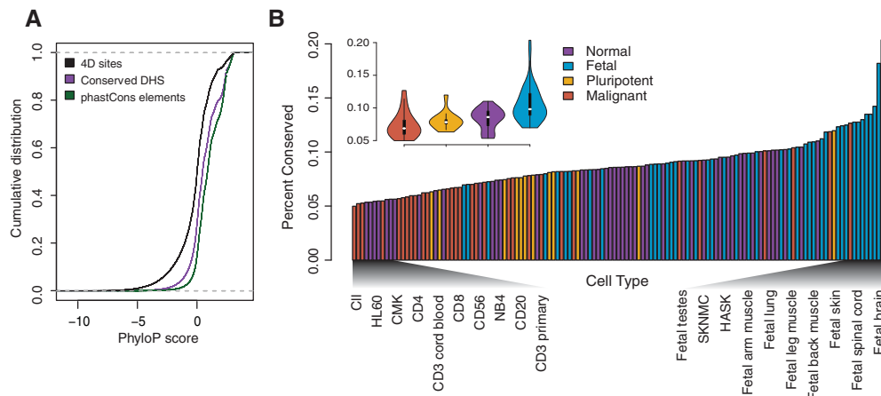
Figure 2. Patterns of conservation vary across cell types. (A) Cumulative distribution of single-base phyloP scores are shown for fourfold degenerate sites, conserved DHSs, and phastCons elements. The dotted gray line indicates a cumulative distribution of zero or one. (B) The proportion of conserved DHSs in each of the 130 cell types, ordered in increasing amounts of conservation. Colors denote four cell type categories: normal (purple), fetal (blue), pluripotent (yellow), or malignant (red). (Inset) Violin plot shows the distribution of the proportion of conserved DHSs for each cell type category. Cell type names at each end of the spectrum are shown for comparison.
