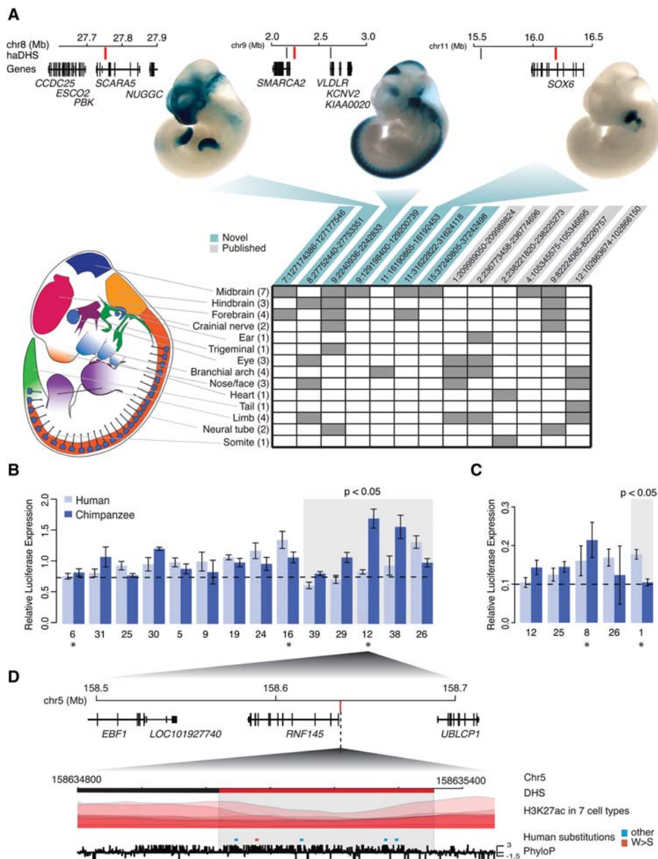
Figure 5. Experimental assays of enhancer activity in haDHSs. (A) A schematic of the transgenic mouse model is depicted. Rows in the table correspond to each embryonic region, and numbers in parentheses indicate how many of the haDHSs were positive in the region indicated. Columns represent the 13 haDHSs that showed enhancer activity, and gray boxes indicate what tissues the haDHS was active in. Three examples of positive assays are shown above, along with a schematic depicting their location relative to nearby genes. The haDHS tested is shown in red, and other haDHSs in the region are shown in black. (B,C) Results from luciferase assays for haDHSs that showed significant enhancer activity in SK-N-MC and IMR90 cells, respectively. Dotted lines indicate the mean relative expression from the negative controls, and the gray box indicates haDHS human and chimpanzee sequences that showed significantly different activity ( P < 0.05 ). Bars, SE. Asterisks below each plot indicate haDHSs that were active in SK-N-MC or IMR90 (other haDHSs were active in similar cell types, such as fetal brain or NHLF). (D) A schematic of the region surrounding haDHS12, which had the largest difference in enhancer activity. The haDHS is located just upstream of the alternatively spliced gene RNF145 . Red substitutions are weak to strong, and all other substitutions are colored in blue. PhyloP scores are also shown across the region. This DHS was partitioned prior to statistical testing into two distinct DHSs. The red portion is human accelerated, and the black portion is not.
