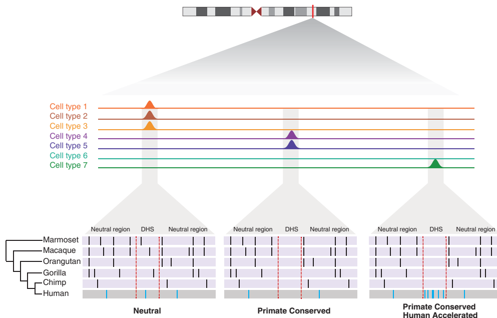
Figure 1. Identifying evolutionarily conserved and accelerated human regulatory sequences. Schematic shows the framework for identifying DHSs that are conserved in primates but accelerated in the human lineage. DHSs appear as peaks of high coverage along the genome and are merged across cell types. An alignment (purple and gray boxes) of six primates is obtained for each DHS and the neutral sequence surrounding them. Black bars represent any sequence that differs from the human sequence, except in the case where all species differ from human, which are represented as blue bars in the human sequence. Dotted red lines indicate the location of the DHS.
