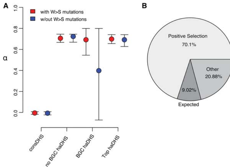
Figure 4. Factors contributing to rate acceleration of haDHSs. (A) Estimates of the proportion of adaptive substitutions, \alpha , and 95% bootstrap confidence intervals for different classes of haDHSs. Red and blue denote estimates that include or exclude weak to strong mutations, respectively. (B) Pie chart summarizing the proportion of substitutions in haDHSs inferred to be influenced by different factors. Expected indicates the proportion of substitutions assuming rates of evolution in the human lineage were the same as that in nonhuman primates; other, substitutions due to other factors such as relaxation of constraint or mutation rate heterogeneity.
