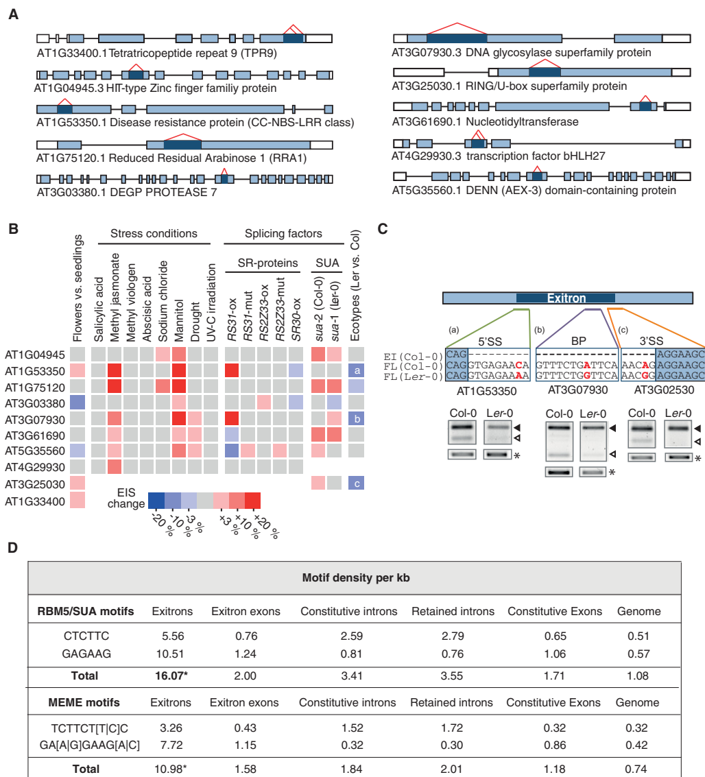
Figure 3. Regulation of exon splicing in Arabidopsis . (A) Structures of EL_{x3} -containing genes tested by RT-PCR in B. Dark blue indicates exon; red caret, exon splicing. (B) Heatmap for EIS in different tissues, stress conditions, splicing factor mutant and overexpression lines, and Col-0 and Ler-0 ecotypes. The coloring represents only significant changes ( P -value \leq 0.1 ). a, b, and c refer to cases described in C. (C) SNPs affect EIS in Ler-0 ecotype. SNPs in the splicing signals are indicated in red. 5'SS, 3'SS, and BP indicate 5' splice site, 3' splice site, and branch point, respectively. RT-PCR products of the full-length (FL) and EI-spliced isoforms (filled and open triangles, respectively) are shown. Ubiquitin was used as a loading control (*). (D) RBM5/SUA motifs and MEME-predicted motifs are enriched in exintrons ( ^* P -value < 0.0001 ).
