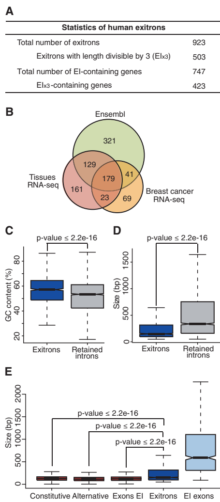
Figure 5. Identification and characterization of human EIs. (A) General statistics of human EIs. (B) Venn diagram of EIs identified by different sources. (C,D) Comparisons of GC content (C) and size distributions (D) of EIs and IRs. (E) Comparison of size distributions of EIs and different types of exons. (C–E) Data presented as Tukey box plots.
