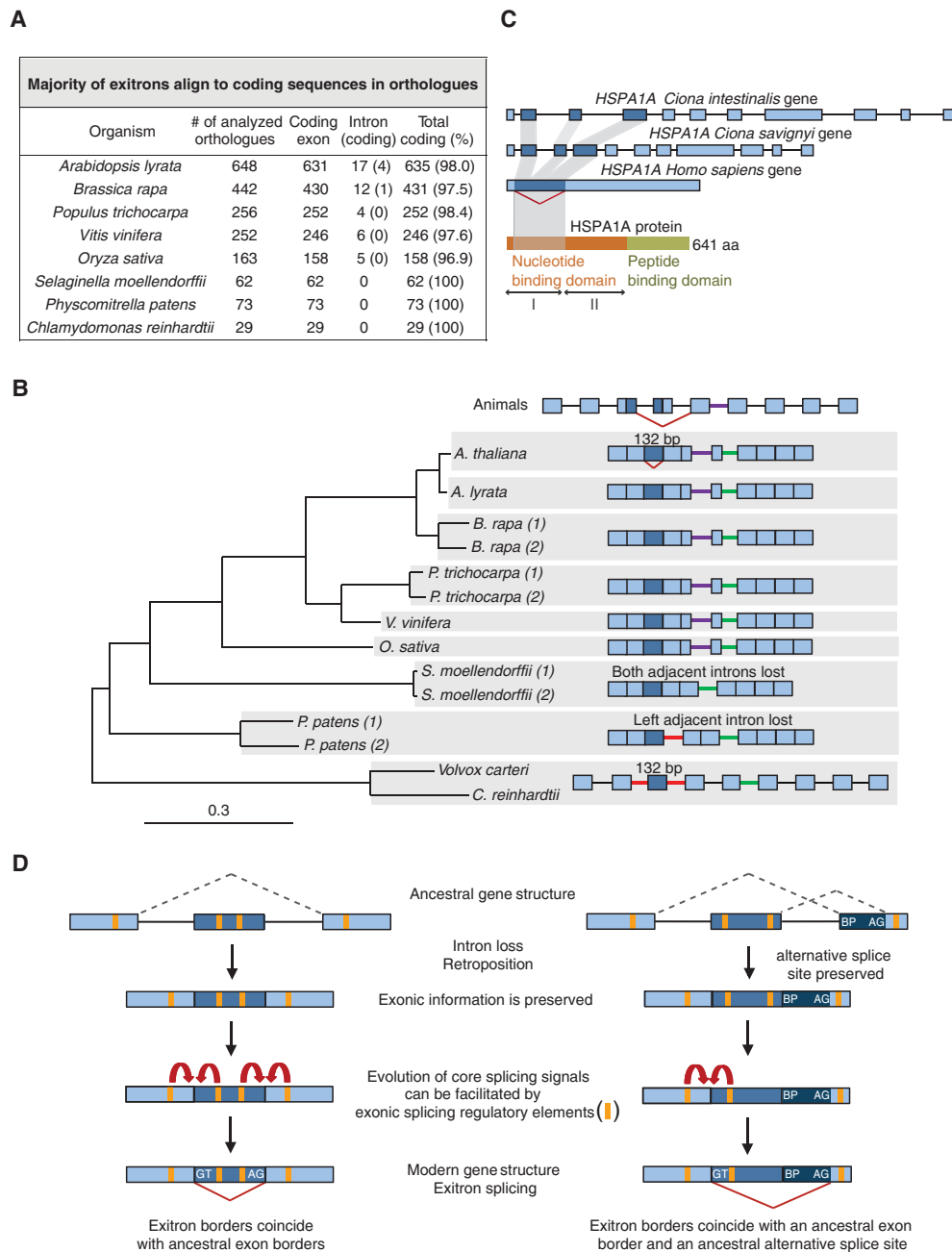
Figure 7. Origin and evolution of EIs. (A) Statistics of EI alignments to plant orthologous sequences. (B) EI evolution in the gene encoding glycine cleavage system T-protein. Phylogenetic reconstruction of intron loss events in different plant species (1 and 2 indicate paralogs). Gene structures are not to scale. Introns at the conserved positions are colored. EI and the homologous sequences are in dark blue. Red carets, EIS and ES events. (C) EI evolution in the intronless human HSPA1A gene. The human EI corresponds to three coding exons in Ciona spp. (D) Evolution of EIS, the “splicing memory” hypothesis. Evolution of a subset of EISs involved loss of introns and retroposition. Upon intron loss, exonic information was preserved. If ancestral regions were subjected to alternative splicing (dashed lines), vestigial exonic splicing regulatory elements present close to the former exon borders could facilitate evolution of core splicing signals and the reestablishment of an AS event in the modern gene by EIS.
