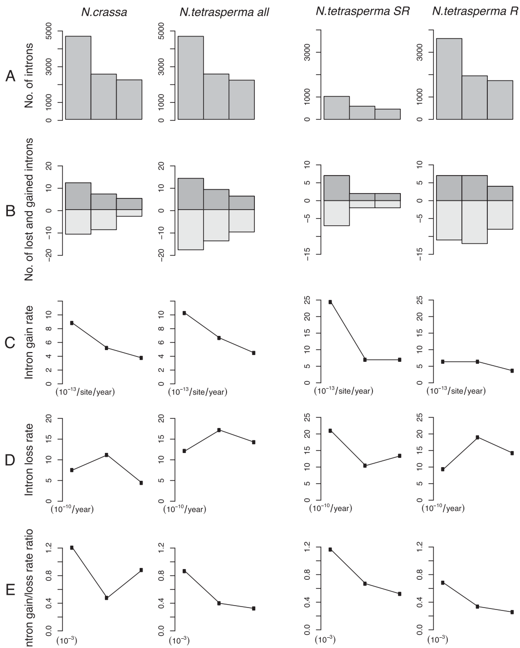
Figure 3. Positional biases of introns and their gains and losses in N. crassa and N. tetrasperma a. Introns are binned into three categories (5', internal, and 3') based on the intron position within a gene, with each category representing one-third of the coding sequence length. In each plot, the bar or point from left to right represents 5', internal, and 3' intron data. Data from N. crassa are presented in the left panel and N. tetrasperma is presented as all intron positions. (SR) Intron positions located within the suppressed recombination region of the mating-type chromosome, and (R) in the normal recombination region of the genome. (A) Number of introns. (B) Number of intron gains and losses since the last common ancestor of N. crassa and N. tetrasperma . Bars above the x-axis represent intron gain number, below, intron loss. (C) Intron gain rate. (D) Intron loss rate. (E) Intron gain/loss rate ratio.
