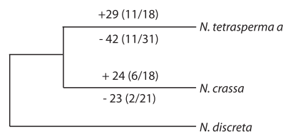
Figure 2. Neurospora phylogenetic tree with numbers of intron gains and losses found at the branches delineating N. tetrasperma and N. crassa . Plus (+) indicates intron gain events, and minus (–) indicates losses. Numbers in parentheses indicate the number of the introns that are located within the region of suppressed recombination of the mating-type chromosome of N. tetrasperma (SR), and in the normal recombination region of the genome (R), as (SR/R). Note that in N. crassa , recombination is not suppressed in the SR region, but numbers are given for comparative purposes.
