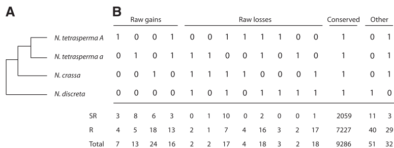
Figure 1. Pattern of intron gains and losses in Neurospora . (A) Phylogenetic relationship of the four Neurospora genomes in this study. (B) Classification of intron presence (1) and absence (0) for the 9495 intron sites. The number of intron sites for each pattern is indicated at the bottom of the figure. SR indicates that the intron position is located within the region of suppressed recombination of the mating-type chromosomes in N. tetrasperma , and R in the normal recombination region of the genome.
