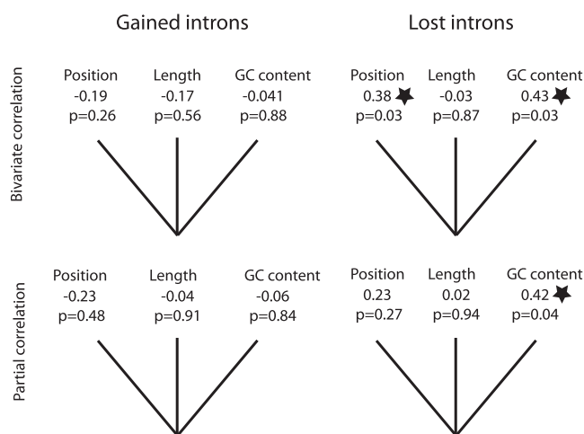
Figure 8. Bivariate and partial correlation test between intron population frequency and intron position, length, and GC content for gained and lost introns. The correlation coefficient and P -value are listed below each category. Tests with statistically significant results are marked with stars.
