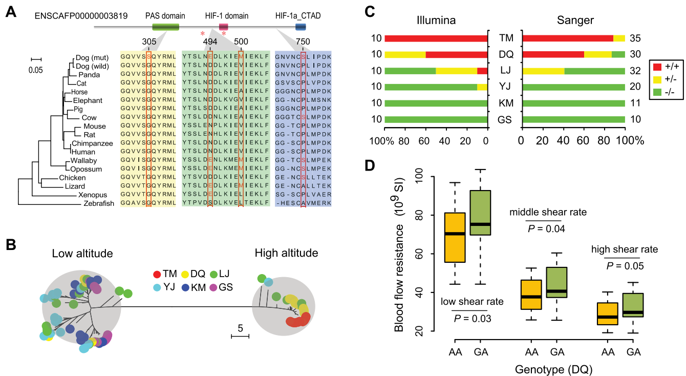
Figure 3. EPAS1 mutations in the coding region. (A) Structural and evolutionary analysis of the four amino acid variants. The protein coordinate is based on Ensembl ID ENSCAF00000003819. The coordinate of NCBI RefSeq XP_531807.2 is slightly different but the variants remain the same. The upper panel shows the Pfam domains of the protein. The orthologous protein sequences from 17 vertebrates are aligned with the mutant residues shown in red. The NJ tree derived from the multiple alignment is shown in the left panel. The red stars indicate two hydroxylation sites (Pro405 and Pro531), which are essential for oxygen sensing (Patel and Simon 2008). (PAS) Per-Arnt-Sim; (HIF) hypoxia-inducible factor; (CTAD) C-terminal transactivation domain. (B) NJ tree of the 8-kb haplotypes comprising the four nonsynonymous mutations. The evolutionary distance is defined as the number of different nucleotides between haplotypes. The haplotypes from high- and low-altitude breeds were grouped into two distinct clades. (C) Percentages of homozygotes and heterozygotes in the six breeds. The mutant and reference alleles are represented by “+” and “-”, respectively. Besides the 60 dogs sequenced with the Illumina technology, additional samples were genotyped with Sanger sequencing. The sample size is shown beside the bars. (D) Association between EPAS1 genotypes (mutant allele, A; reference allele, G) and blood flow resistance in DQ. The blood flow resistance was measured at different shear rates. In the boxplot, the line within the box defines the median; the ends of the boxes define the 25th and 75th percentiles; and the error bars define the 10th and 90th percentiles. The ANOVA F -test was performed, taking the age as covariant.
