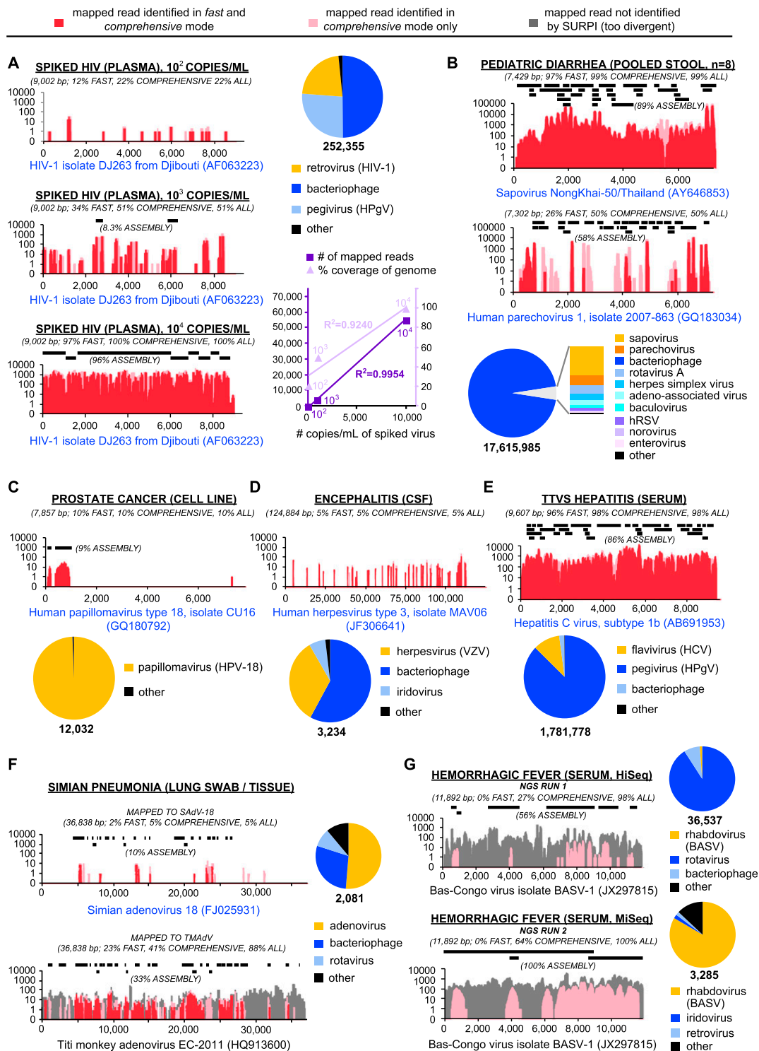
Figure 5. The SURPI pipeline correctly identifies viral species in clinical NGS data sets. Data sets corresponding to clinical samples or sample pools harboring target viral pathogens were analyzed using SURPI. Pie charts show detected viruses derived from the output summary tables. Target viruses are color-coded in yellow or orange; other viruses are color-coded ranked by their relative abundance from shades of blue, followed by shades of purple. Coverage maps of the “best hit” viral genome in fast mode (red) and comprehensive mode (pink, overlaid by red) display automated SURPI output corresponding to the detected target viral genome (blue text). The read coverage (y-axis, log scale) and de novo assembled contigs (black lines) are plotted as a function of nucleotide position along the genome (x-axis). Percent coverage achieved using SURPI in fast mode (“FAST”), in comprehensive mode (“COMPREHENSIVE”), and by de novo assembly (“ASSEMBLY”), as well as the actual coverage from all reads in the data set (“ALL”) are shown. (A) Coverage plots of HIV-1 spiked at titers of 10 2 –10 4 copies/mL. The number of mapped reads and percent coverage are plotted against the viral copy number ( inset ). Coverage plots of SaV and HPeV-1 (B), HPV-18 (C), HHV-3 (D), and HCV-1b (E). (F) Coverage plot mapping SURPI-classified genus-level Mastadenovirus reads (red/pink) to the SAdV-18 genome, or Mastadenovirus reads (red/pink) and all specific TMAdV reads (gray) to the TMAdV genome. (G) Coverage plots mapping SURPI-classified family-level Rhabdoviridae reads (pink) or all specific BASV reads (gray) to the BASV genome.
