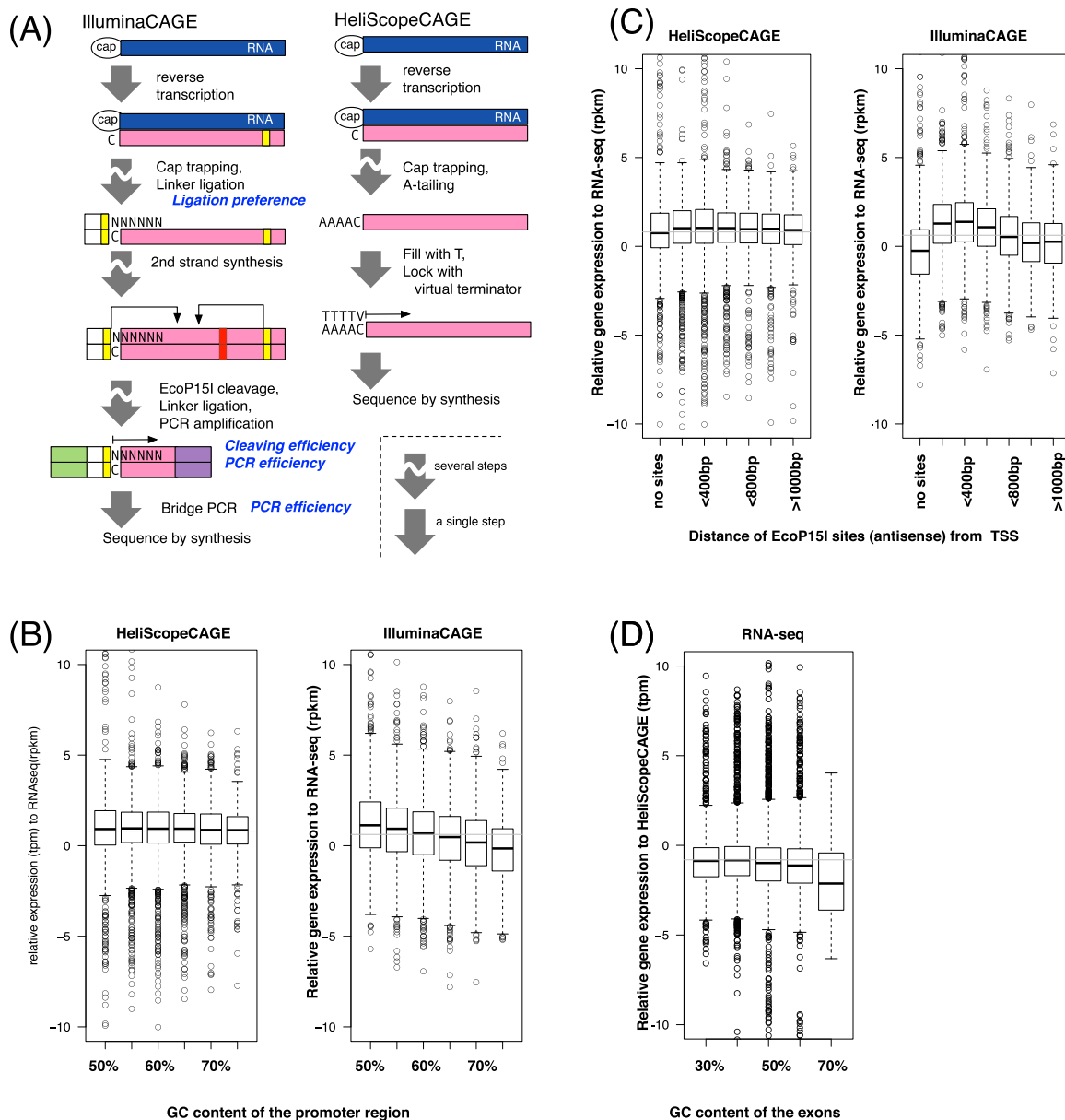
Figure 4. Systematic bias at the gene level. (A) Schematic view of the CAGE platforms. Blue box indicates RNA; pink box, DNA; yellow box, EcoP151 sites; red box, internal EcoP151 sites; and green and purple boxes, 5' and 3' linkers. Text in blue suggests potential causes of gene quantification bias. (B) Relative expression of the CAGE profiles against RNA-seq quantification, according to GC content within 500 bp from RefSeq TSS. (C) Relative expression of the CAGE profiles depending on the presence of EcoP151 sites on an antisense strand to the gene orientation. (D) Relative expression of the RNA-seq profiles against HeliScopeCAGE quantification, according to GC content of the exons.
