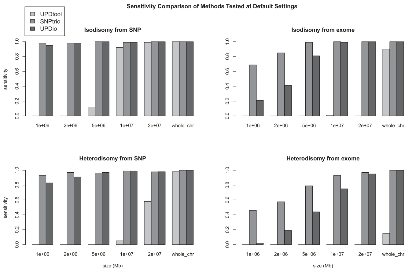
Figure 3. Sensitivity comparisons. Simulations were performed to measure the sensitivity of detecting introduced UPD events from SNP and exome data, ranging in size from 1 Mb to chromosomal.
