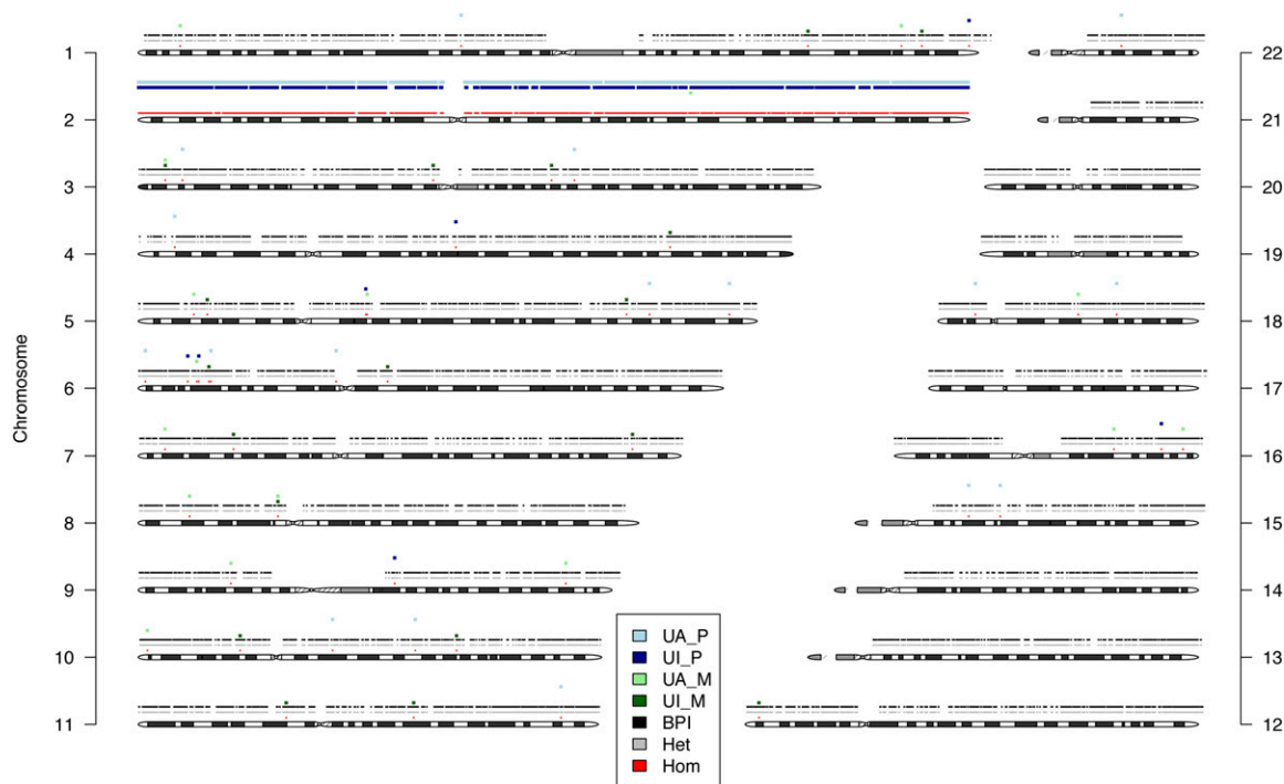
Figure 7. UPD example plot. A plot of QC-passing proband genotypes on each autosome. The position and color reflect zygosity (homozygous, heterozygous) and informative state (biparental inheritance, maternal isodisomy, maternal heterodisomy or isodisomy, paternal isodisomy, paternal heterodisomy or isodisomy). The figure displays each chromosome ideogram. Each chromosome has an x-axis (chromosome position) and y-axis (zygosity, and informative event type). In this case, the UPD event for chromosome 2 is depicted with a mixture of dark-green points (maternal isodisomy) and light-green points (maternal isodisomy or maternal heterodisomy). The zygosity row demonstrates homozygosity along the entirety of the chromosome, reflecting the complete isodisomy.
