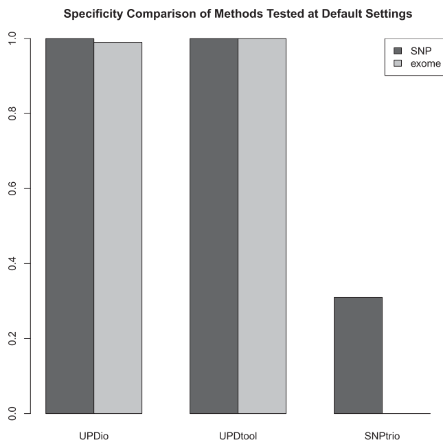
Figure 4. Specificity comparisons. Simulations on normal SNP and exome samples were compared to measure the proportion of samples without UPD detections.
