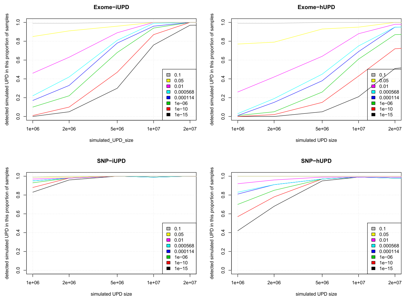
Figure 2. Sensitivity of UPD detection simulations. Simulations to assess sensitivity of UPD detections at different sizes, from different data sources. (iUPD) Isodisomy; (hUPD) heterodisomy.
