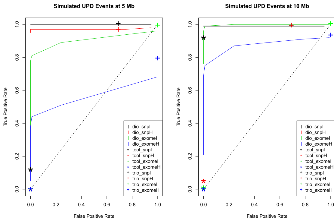
Figure 5. Receiver operator characteristic curve comparing UPD detection accuracy. Accuracy of UPD detection at different simulated UPD sizes. (dio) UPDio; (tool) UPDtool; (trio) SNP trio.
