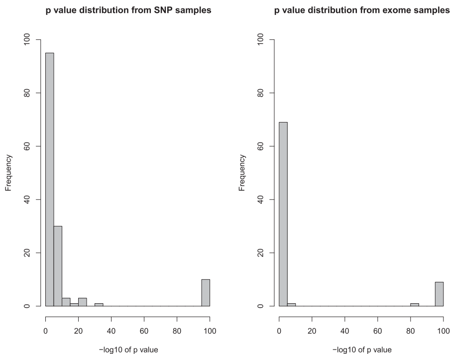
Figure 6. DDD UPD P -value distributions. Distribution of the -\log_{10} P -values for UPD detections from different data sources, with or without CNV data. Presence of sample-specific CNV data increases the proportion of extremely significant events and decreases the proportion of marginally significant events. P -value minimum truncated to 1 \times 10^{-100} .
