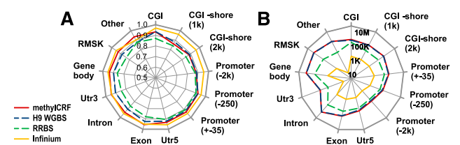
Figure 5. Comparison between MethylC-seq and methylCRF and other methylation assays. (A) Concordance of methylCRF, BS-seq, RRBS, and Infinium array with MethylC-seq within a 25% window broken out by annotated genomic features. Note that BS-seq (H9) is a female sample, while MethylC-seq (H1) is a male sample. Only CpGs in common were compared. (B) The number of CpGs used for each comparison on a \log_{10} scale.
