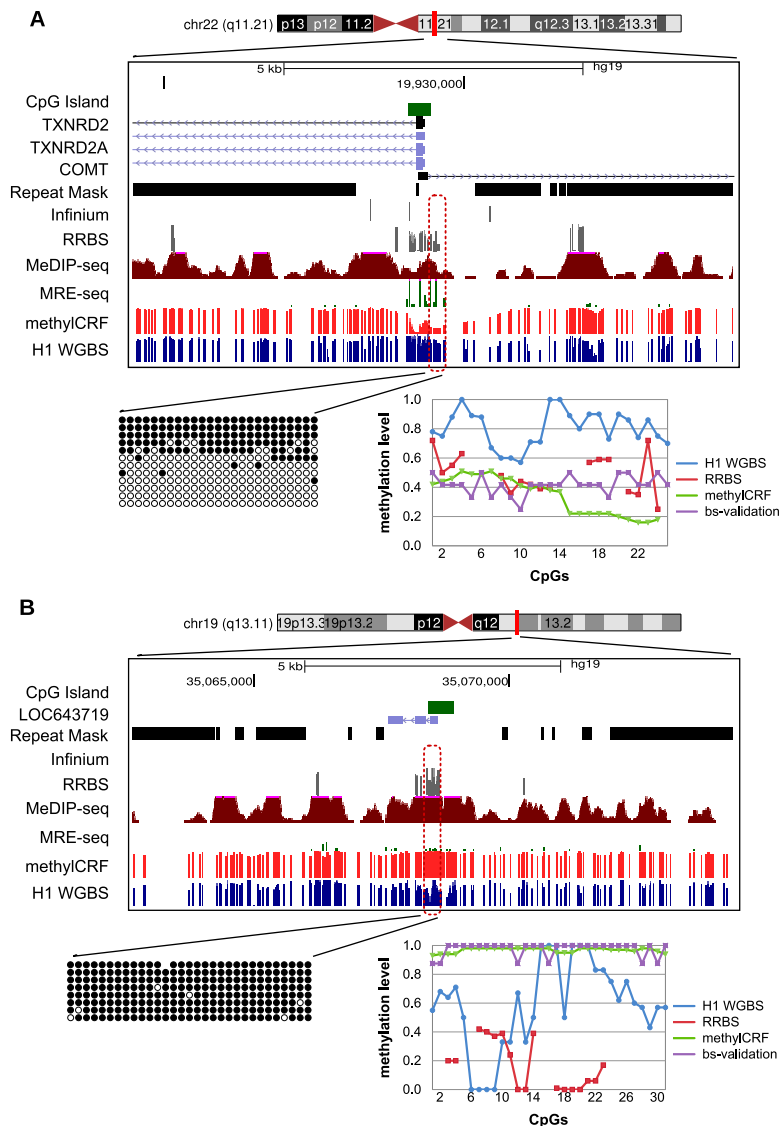
Figure 9. Experimental validation of regions where there is discordance between MethylC-seq and methylCRF. Genome Browser view and site-specific bisulfite sequencing validation for each region (○ unmethylated CpG; ● methylated CpG). The line graph shows the methylation levels estimated by MethylC-seq, RRBS, bisulfite validation, and methylCRF. (A) chr22: 19929336–19929659; MethylC-seq predicted on average a methylation level of 80% methylated, while methylCRF and bisulfite validation agreed on a level of 40% methylated. (B) chr19: 35068305–35068683; MethylC-seq predicted on average a methylation level of 60% methylated, while methylCRF and bisulfite validation agreed that the region is more than 90% to completely methylated.
