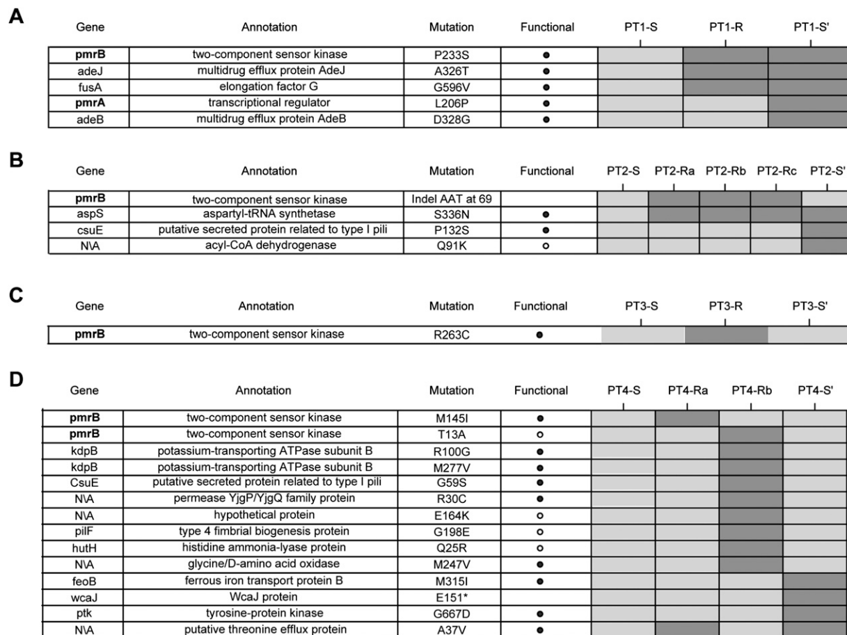
Figure 2. Genome-wide single-nucleotide variants in longitudinal patient isolates. (A–D) Rows in each table represent all nonsynonymous mutations identified across the genomes of isolates derived from patients 1 through 4. Isolates from each patient are shown in temporal order, in the columns of the corresponding patient's heatmap. Dark/light gray boxes in the heatmap represent the presence/absence of mutations in patient isolates. The pmr genes appear in boldface, to emphasize their mutation in the resistant isolates from each patient. The putative functional impact of mutations was predicted using SIFT. Note that for PT3-S' unique mutations are not shown, as this is a different strain type from PT3-S and PT3-R and, therefore, has several hundred unique variants.
