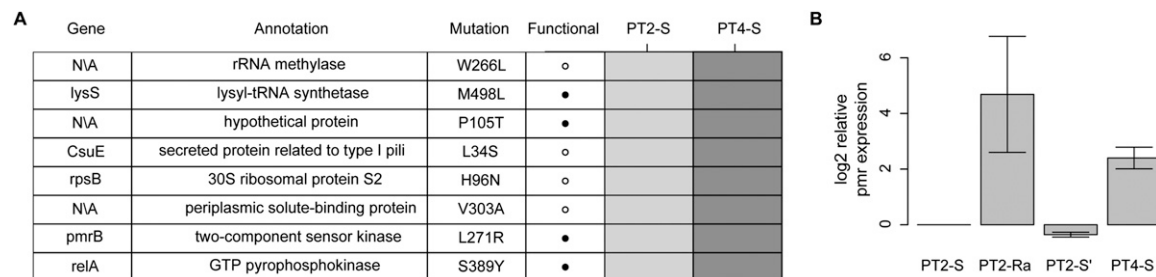
Figure 4. Initial isolate from patient 4 has elevated pmr expression. (A) Rows in the table represent all nonsynonymous mutations in nonrecombinant regions identified between the initial isolates of patients 2 (PT2-S) and 4 (PT4-S). Dark/light gray boxes in the heatmap represent the presence/absence of mutations in patient isolates. The pmr gene mutation is bolded to emphasize its hypothesized role in colistin resistance of PT4-S. (B) The expression of the pmr transcript relative to PT2-S is shown for PT2-R, PT2-S', and PT4-S. The expression values are the mean and standard error for three replicates
