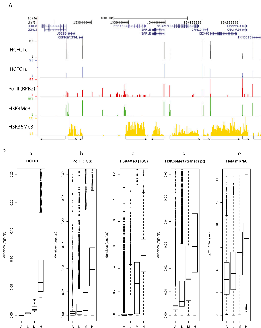
Figure 2. HCFC1 peaks correlate with sites of active promoters. (A) UCSC Genome Browser shot showing a typical distribution of HCFC1 C and HCFC1 N binding sites together with Pol II, and H3K4Me3 and H3K36Me3 modified histones. (B) TSS regions (−250 to +250 bp from TSSs) were split into four categories according to the density of sequence tags (number of tags centered to the fragment length as in Fig. 1E divided by the number of base pairs, i.e., 500) for HCFC1 C (panel a). (A) Absent (density = 0, 6270 transcription units); (L) low density (density > 0 and ≤0.004, 4806 transcription units); (M) medium density (density > 0.004 and ≤0.03, 7902 transcription units); (H) high density (density > 0.03, 3417 transcription units). The sequence-tag densities for Pol II (panel b) and H3K4Me3 (panel c) at promoter regions and H3K36Me3 (panel d) within transcribed regions are shown for each category. The distribution of transcript abundance in log 2 of transcripts in HeLa cells is shown for each category (panel e). The results are displayed as boxplots.
