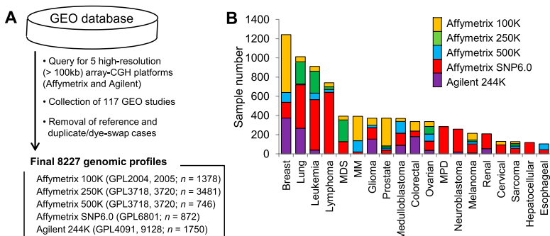
Figure 1. Compilation of large-scale cancer genome copy number profiles. (A) A schematic of data collection is shown. Five high-resolution, array-CGH platforms used are listed with the corresponding GEO accession ID (GPL) and the number of associated samples. (B) Major tumor types (>100 samples for each type) are shown with their sample numbers with respect to the five platforms. (MDS) Myelodysplastic syndrome, (MM) multiple myeloma, (MPD) myeloproliferative disorder.
