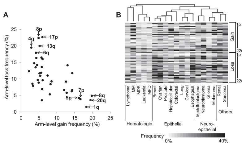
Figure 2. Overview of chromosomal arm-level alteration frequency. (A) A scatter plot shows the arm-level alteration frequency measured across the entire data set ( n = 8227 ). The top five most frequently gained or lost chromosomal arms are marked. Size-adjusted arm-level alteration frequencies are separately shown in Supplemental Figure S4. (B) Hierarchical clustering using the arm-level alteration frequency largely segregates 19 tumor types into three clusters of hematologic, epithelial, and neuroepithelial origins (from left to right). The heat map shows the frequency of chromosomal copy gains (above) and losses (below), ordered from 1p to 22q.
