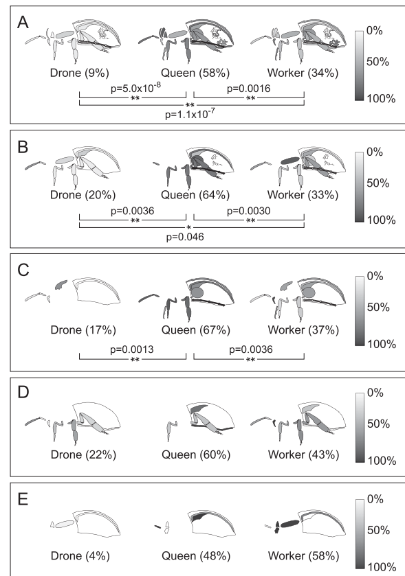
Figure 5. Caste and organ distribution of immunity proteins. (A) PPO, (B) PGRP-S3, and (C) GGBP 1-2 expression is significantly higher in queens compared with the other castes. Overall expression levels of the antimicrobial peptides hymenoptaecin (D) and defensin (E) are not different ( P > 0.1 ), except that drones express far less defensin than queens or workers. Relative levels across each organ shown on a grayscale. Whole-body averages are shown in parentheses; (*) P < 0.05 , (**) P < 0.01 .
