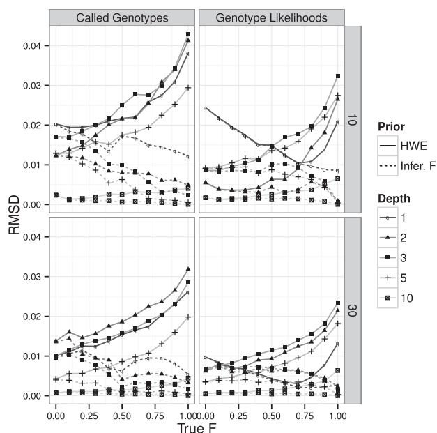
Figure 3. Effect of the inbreeding coefficient on SFS estimation. Performance of SFS estimation from called genotypes ( left column ) and the Nielsen et al. (2012) method from GL and assuming inbreeding ( right column ), on a sample size of 10 (first row) and 30 (second row) individuals and 10,000 variable sites simulated with a 0.5% error rate. Line styles and symbols represent different simulated sequencing coverages. Line types depict the level of inbreeding assumed in the priors: F = 0 (HWE; filled) or inferred value of F (Infer. F; large dashes).
