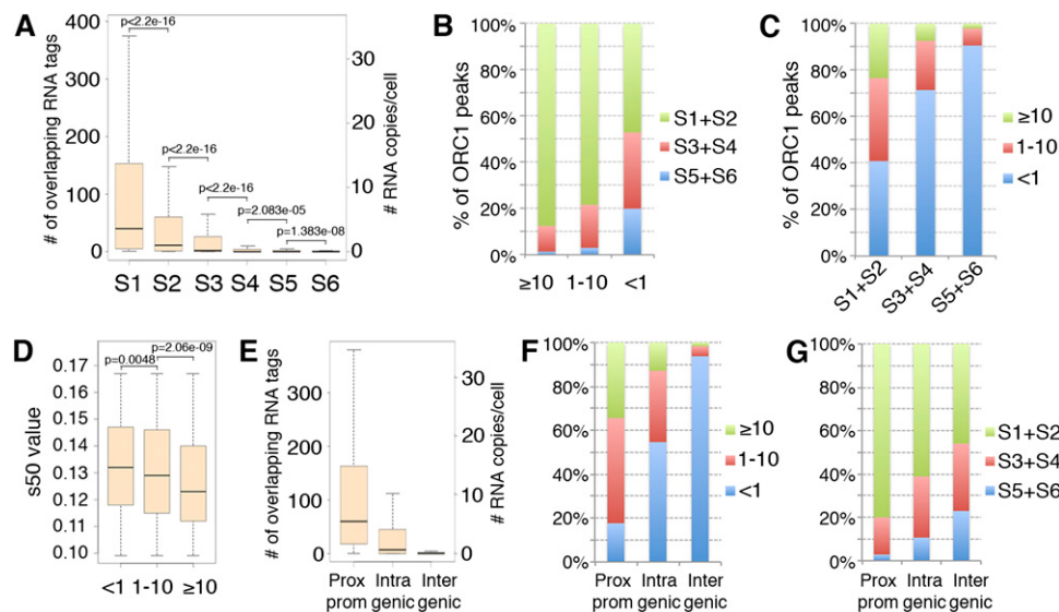
Figure 6. Transcription levels at ORC1 peaks correlate with replication timing. (A) Boxplots of the transcription levels measured at ORC1 peaks replicating in the S1–S6 windows. (B) Frequency of early (S1 + S2), middle (S3 + S4), or late (S5 + S6) replicating ORC1 peaks within groups with homogenous expression ( < 1 , 1–10, or \geq 10 RNA copies/cell). (C) Frequency of ORC1 peaks with different transcription levels ( < 1 , 1–10, or \geq 10 RNA copies/cell) within groups of ORC1 sites homogeneous for replication timing. (D) Boxplots of the s50 values of ORC1 peaks with different transcription levels ( < 1 , 1–10, or \geq 10 RNA copies/cell) mapping within very-early-replicating (S1) inverted-V apexes. (E) Boxplots of the transcription levels measured at the ORC1 peaks mapping within proximal promoters of known genes, intragenic, or intergenic regions, as indicated. (F) Frequency of ORC1 peaks with different transcription levels ( < 1 , 1–10, or \geq 10 RNA copies/cell) for each genomic location, as indicated. (G) Frequency of early (S1 + S2), middle (S3 + S4), or late (S5 + S6) replicating ORC1 peaks for each genomic location, as indicated.
