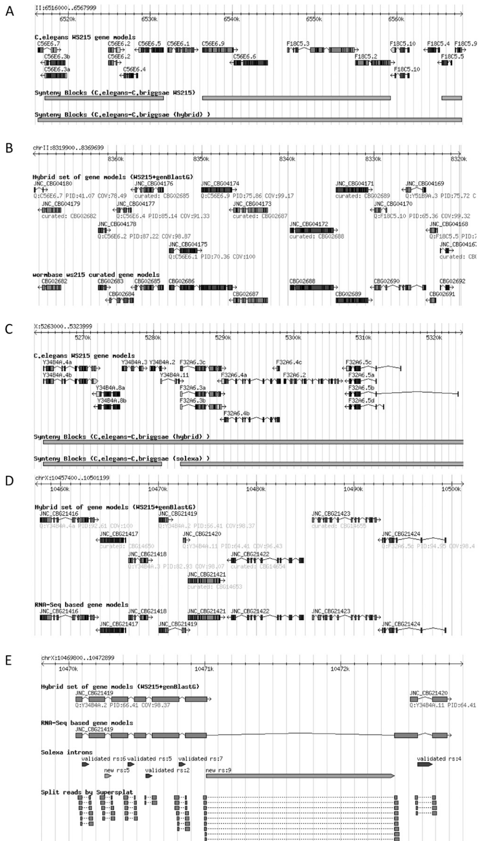
Figure 4. Gene model revision and synteny analysis. (A) genBlastG-based C. briggsae gene model revision enables the discovery of larger synteny blocks between C. elegans and C. briggsae . Three small synteny blocks were merged into one single larger synteny block that contains all their adjacent synteny blocks. (B) Four C. briggsae gene models, which were revised or discovered in the genBlastG-based gene model revision, are shown at the synteny block break points. (C) A synteny block between C. elegans and C. briggsae is broken down into two smaller synteny blocks. (D) Two hybrid gene models were merged to form a single gene model based on an RNA-seq Illumina intron. (E) RNA-seq evidence supports the merger of two hybrid C. briggsae gene models into a single gene model. (RS) Number of supporting reads.
