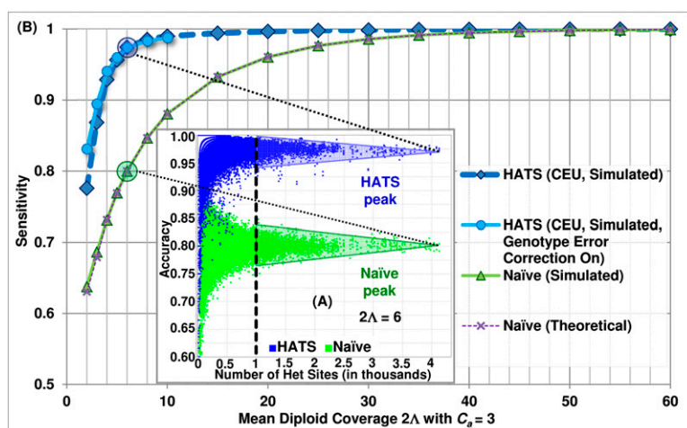
Figure 1. Accuracy example and sensitivity of HATS and the naive method from simulations, European (CEU) training data set. (A) Accuracies of each sample trial ( 2\lambda_j = 6 , C_a = 3 ). Each point in the embedded, raised-dot plot represents the accuracy for a particular amplicon a in sample j per trial. As the number of heterozygous sites in a increases, the accuracies converge to a peak for the naive method and a peak for HATS. We set the threshold \nu to 1000 and use k -means clustering to determine the centroids for each peak. The centroid for the naive model resides at \sim 0.80 , which is assigned as the sensitivity for the naive method for parameter values ( 2\lambda_j = 6 , C_a = 3 ). The centroid for HATS exists at \sim 0.975 . (B) Method sensitivities. This figure displays the simulation sensitivity results for HATS (with Genotype Error Correction [GEC] turned on or, by default, off) as well as for the naive method. The naive theoretical curve is included for comparison purposes, illustrating that the naive results can, indeed, be calculated theoretically. Note that it takes up to diploid coverage of 45 until the naive method can match the performance of HATS. The GEC mode noticeably improves performance at very low coverage levels for HATS. The training data set was obtained from the 1000 Genomes Project ( http://www.1000genomes.org/ ).
