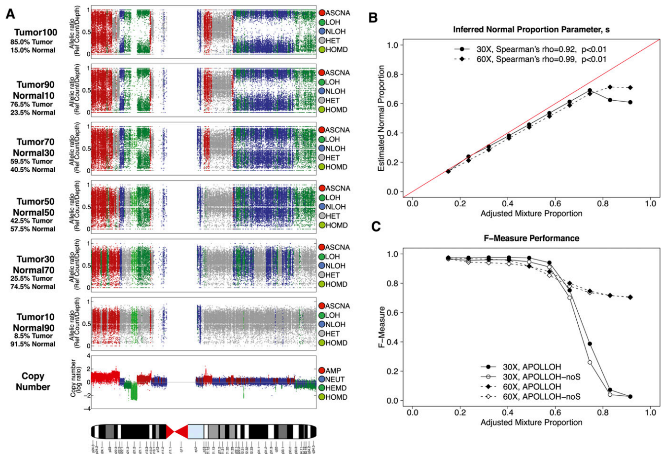
Figure 4. Tumor-normal sampling admixture experiment. Nine mixture proportions generated by sampling reads from the tumor and normal BAM files were analyzed (see Methods). (A) APOLLOH results are shown for chromosome 9 of mixture proportions of 0.09, 0.26, 0.43, 0.60, and 0.77 tumor reads sampled to 30 \times . (Tumour100) Results from the original tumor sample. (B) The normal proportion parameter s inferred by APOLLOH was significantly correlated (Spearman's \rho = 0.92 ) with the mixture proportions of 0.1–1.0 (increments of 0.1) at 30 \times and 60 \times . (C) The F-Measure performance of APOLLOH and APOLLOH-noS (not accounting for normal contamination) for 30 \times and 60 \times admixtures was evaluated using Affymetrix SNP6.0 data as ground truth.
