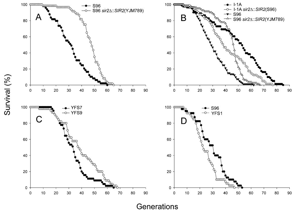
Figure 3. Cumulative survival curves. (A) The RLSs of 49 cells of strain S96 and 60 cells of strain S96 sir2Δ::SIR2(YJM789) were determined. The mRLS of S96 was 31.7 generations, and for S96 sir2Δ::SIR2(YJM789) it was 46.9 generations. The difference in RLS was significant ( P < 5 \times 10^{-6} ). (B) The RLS of 81 cells each was determined. For line I-1A, the mRLS was 49.5 generations; for strain I-1A sir2Δ::SIR2(S96) , it was 41.6. The difference in RLS was significant ( P = 0.0079 ). For S96, the mRLS was 30.7 generations, and for S96 sir2Δ::SIR2(YJM789) it was 43.7 generations. The difference in RLS was significant ( P < 5 \times 10^{-6} ). I-1A is the recombinant line with the longest RLS. (C) The RLS of 45 cells each was determined. For strain YFS7 (YJM789 background with RDN1 from YJM789) the mRLS was 33.8 generations, and for strain YFS9 (YJM789 background with RDN1 from S96) it was 40.0 generations. The difference in RLS was significant ( P = 0.030 ). (D) The RLS of 40 cells each was determined. For strain S96, the mRLS was 29.8 generations, and for strain YFS1 (S96 background with RDN1 from YJM789) it was 24.6 generations. The difference in RLS was significant ( P = 0.032 ). The x-axis shows the RLS in generations and the y-axis shows the percentage of surviving cells.
