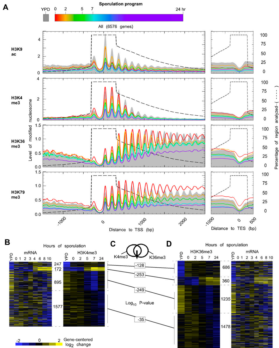
Figure 4. Nucleosomal and histone modification distribution around genomic features. (A) Distributions of indicated H3 modification states (rows of panels) are plotted around the TSS and TES for all genes. Traces reflecting different time points in the sporulation program are color-coded as indicated, and further described in Figure 1A. Total tag counts in each sample were scaled to reflect the bulk distribution, measured by immunoblotting (Supplemental Fig. S8). Consequently, the plots reflect the level of modified nucleosomes, not the density of modification per H3 nucleosome. The H3K79me3 antibody may have significant cross-reactivity with me2. Cluster plots for H3K4me3 (B) and H3K36me3 (D) changes on a gene-by-gene basis show that both H3K4me3 and H3K36me3 are linked with transcription. In contrast to A, the total tag count for all samples (H3, H3K4me3, and H3K36me3) were normalized to be equal. Each row included gene-centered log 2 transformed H3K4me3/H3 ratios (from the 0- to 500-bp region relative to TSS for H3K4me3 and the 300- to 1000-bp region relative to TSS for H3K36me3) for all six time points. Gene-centering means that the average of each row is set to zero. All genes were arranged by k -means clustering ( k = 5). The number of genes in each cluster is indicated. One cluster was omitted as it displayed no changes. Corresponding changes in mRNA levels (Primig et al. 2000; Williams et al. 2002) are shown. Levels of mRNA were gene centered and log 2 transformed. (C) \chi -tests between clusters of H3K4me3 and H3K36me3 suggest that two methylation marks are significantly coincident. Venn diagram relating the overlap of clusters 1–4 in B with the corresponding clusters in D. Values below the Venn diagram reflect log 10 P -values ( \chi -test) of the overlapping membership.
