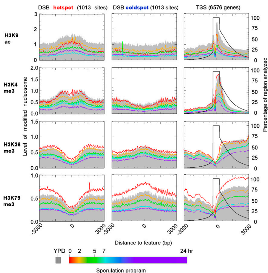
Figure 5. Distribution of nucleosomes and histone modification states around meiotic recombination hot and cold spots. The distribution of nucleosomal tags and levels of the indicated modification states around double-strand break (DSB) hotspots and cold spots (Borde et al. 2009) during the sporulation program are displayed in the first two columns of graphs. To assess nucleosome densities, plots should be compared against Figure 2A. The third column displays tag distributions around the TSS as shown in Supplemental Figure S9B for comparison, but is highly smoothed to achieve the lower resolution of the DSB sites.
