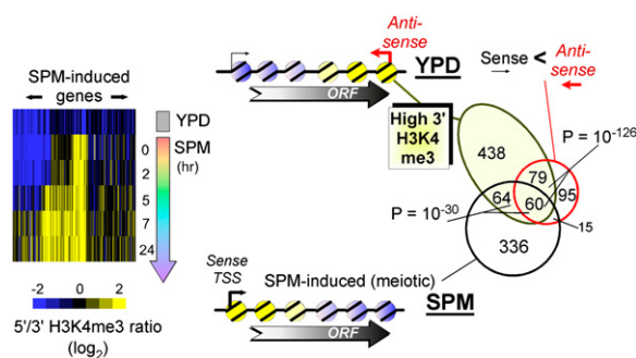
Figure 6. H3K4me3 provides a signature of repressive antisense transcription. The ratio of H3K4me3 density at the 5' end to the 3' end of every gene was calculated. The intersecting genes of meiotic specific genes and the genes having \log_2 ratios that were negative at rich media were selected and k -means ( k = 3 ) clustered ( n = 124 ). The cluster plot is shown on the left and is turned 90° from the normal orientation. Genes are columns, rows are time points, and blue/black/yellow color scale reflects the \log_2 5'/3' ratio. The top Venn diagram shows the overlap between these genes and those that produce greater antisense than sense transcription (Parkhomchuk et al. 2009). The bottom Venn diagram shows the overlap with sporulation-induced genes (Chu et al. 1998). \chi -test P -values are shown.
