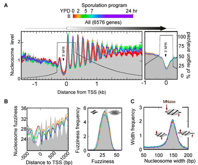
Figure 1. Nucleosome organization around genes throughout sporulation. (A) Composite nucleosome distribution traces for six time points in the meiosis/sporulation program are color-coded as indicated. Nucleosome midpoint density is represented by sequencing tag counts from cross-linked, MNase-digested, H3 immunoprecipitated, and gel-purified samples. Distributions were normalized such that the total tag count in each sample was equal. Tag counts are distributed about 6576 transcript start (TSS) and end (TES) sites in 3-bp bins and 15-bp bins, respectively, and smoothed via a three-bin moving average. The percentage of regions analyzed is indicated by the black trace and covers a minimum of \pm 300 bp from the TSS or TES and a maximum of 300 bp from the next TSS or TES. Bin counts were normalized to the number of regions represented in each bin. (B) Nucleosome fuzziness was taken to be the standard deviation of tag locations for each nucleosome. The average fuzziness per bin was determined, then plotted as described in A. (Right) A frequency distribution of nucleosome fuzziness at various meiotic time points. Color codes are as in A, except that YPD is represented by a black trace. (C) Frequency distribution of nucleosomal widths (distance between the W/+ and C/- MNase-digested borders).
