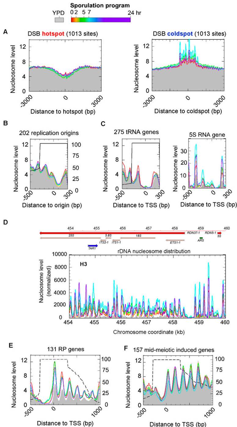
Figure 2. Nucleosome organization around genomic features throughout sporulation. (A–F) Nucleosomal midpoint tags were distributed around the indicated number of genomic features as described in Figure 1, except that bins were 15 bp. Percentages of regions analyzed are on the right.
