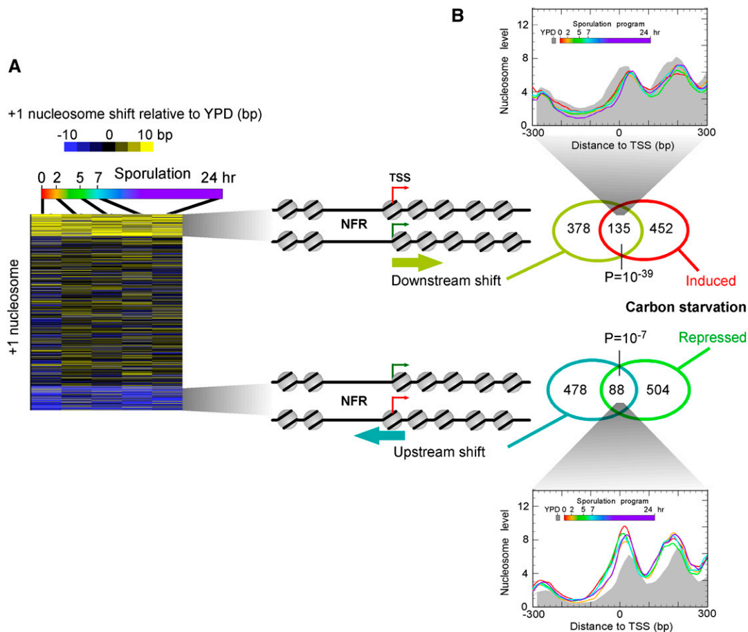
Figure 3. +1 nucleosome shift is linked with carbon starvation regulation. (A) +1 nucleosome midpoint distances from the position found in YPD were calculated for each gene (rows) at all time points (columns) and displayed as a cluster plot. Three distinct groups were identified by k -means clustering. Distances shifted downstream in a positive direction are color-coded yellow. Upstream shifts are colored blue. Equivalent shifts were evident across the genic nucleosomal arrays. (B) Venn diagram and \chi -test are shown for the overlap of the indicated cluster of genes and those genes most up- or down-regulated (as indicated) upon carbon starvation (Bradley et al. 2009). Composite nucleosome distributions around the TSS are shown for the set of intersecting genes.
