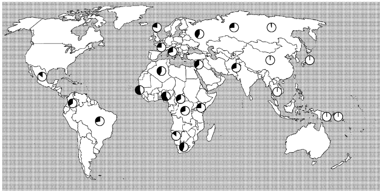
Figure 8. Global genome-wide distribution of alu18507_9 polymorphisms. Allele frequency as determined by PCR of 1054 samples from 52 HGP populations. Insertion polymorphism frequency (black portion of the pie chart) for alu18507_9 is depicted.
