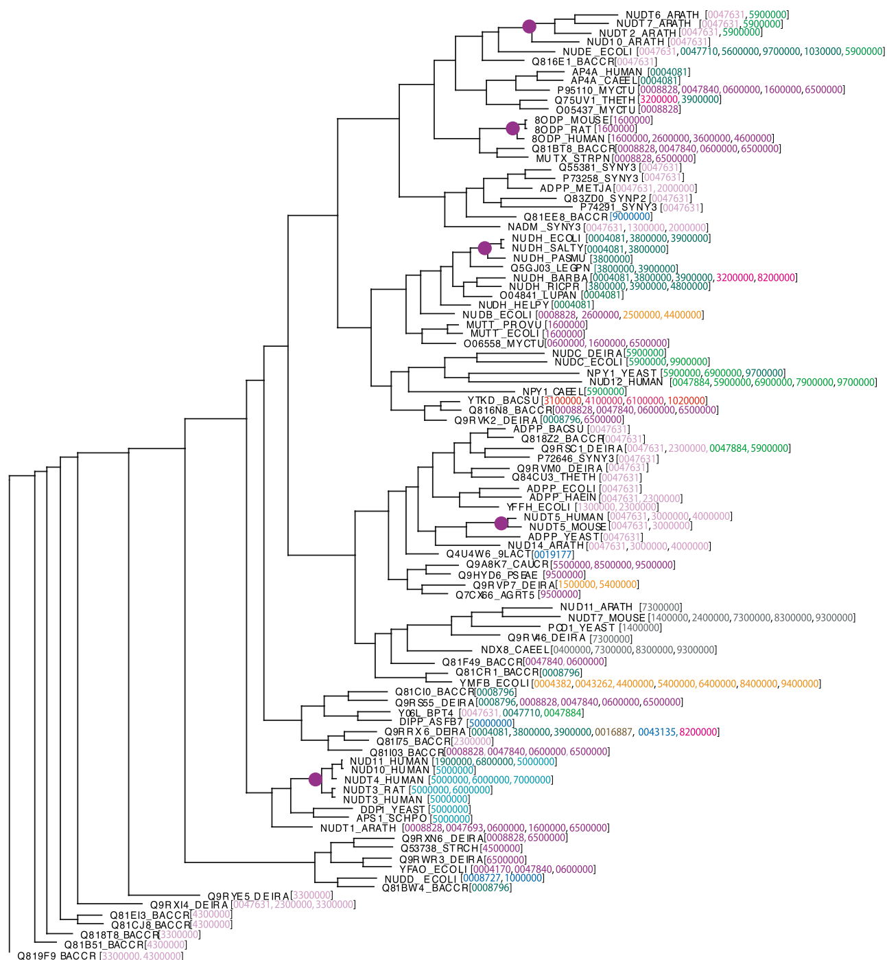
Figure 4. A reconciled phylogeny of the experimentally characterized hydrolase proteins found in the Nudix family. The colored numbers in brackets after the protein name represent a clustering of the proteins into their biological functions, determined from our own literature search and described in more detail in future work. The purple dots represent clades that have >95% bootstrap support.
