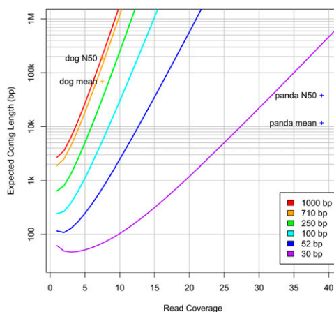
Figure 3. Expected average contig length for a range of different read lengths and coverage values. Also shown are the average contig lengths and N50 lengths for the dog genome, assembled with 710-bp reads, and the panda genome, assembled with reads averaging 52 bp in length.
