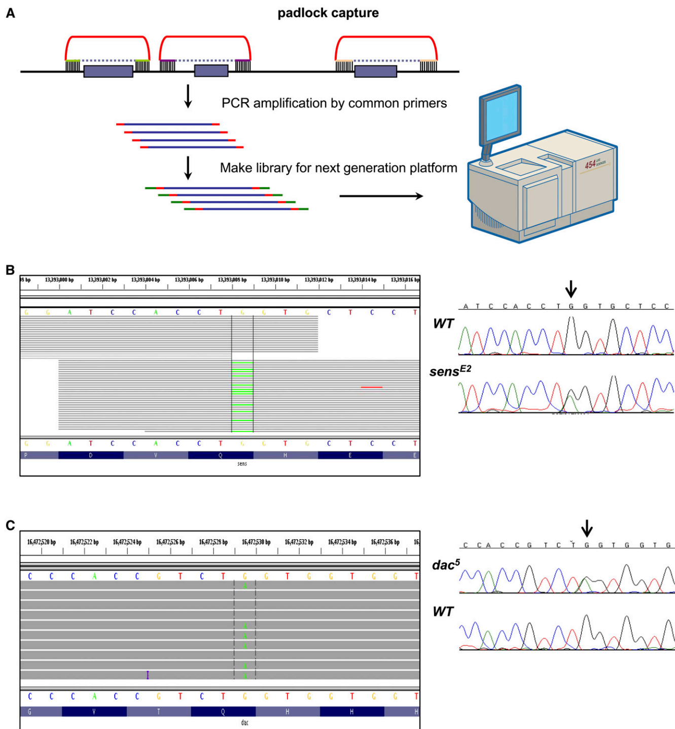
Figure 1. Two known mutations were detected using padlock capture sequencing. (A) Flowchart of mutation detection by padlock capture and next-generation sequencing technologies. Padlock capture technology requires probes that contain two target-specific capturing arms (green) connected by a common linker (red). The unique targeting arms of individual targeting oligonucleotides are designed to hybridize immediately upstream and downstream from each exon (purple bars) of interest. Hybridization to genomic DNA is followed by an enzymatic gap filling and ligation step, such that a copy of the sequence of interest is incorporated into a circle (purple dashed line). Then the enriched DNA is PCR amplified and is used to prepare libraries for the next-generation platform sequencing. (B) sens E2 and (C) dac 5 mutation detection. Reads alignment at the mutation is shown between the vertical lines. Each read is drawn as a gray line, and bases that are different from the reference are colored. Sanger sequencing is conducted to confirm the mutation with the heterozygous mutated base indicated by the arrow.
