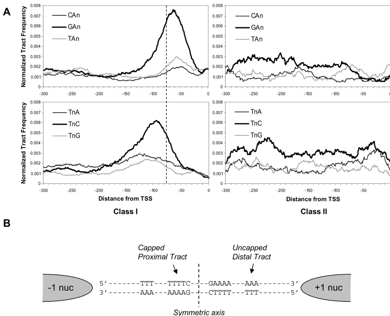
Figure 6. 5' G:C capping splits poly(dA:dT) tracts into subpopulations proximal and distal to the symmetric axis. (A) Frequencies of poly(dA:dT) tracts ( n = 4 ) with different 5' capping bases were computed in class I and class II promoters. Frequencies represented on the vertical axis are numbers of motifs per promoter per base smoothed across a 21-bp window. Bold black curves represent 5' G:C capping. (B) Schematic representation of the data from (A) showing a hypothetical class I promoter with 5' G:C-capped and -uncapped poly(dA:dT) tracts arranged across the symmetric axis.
