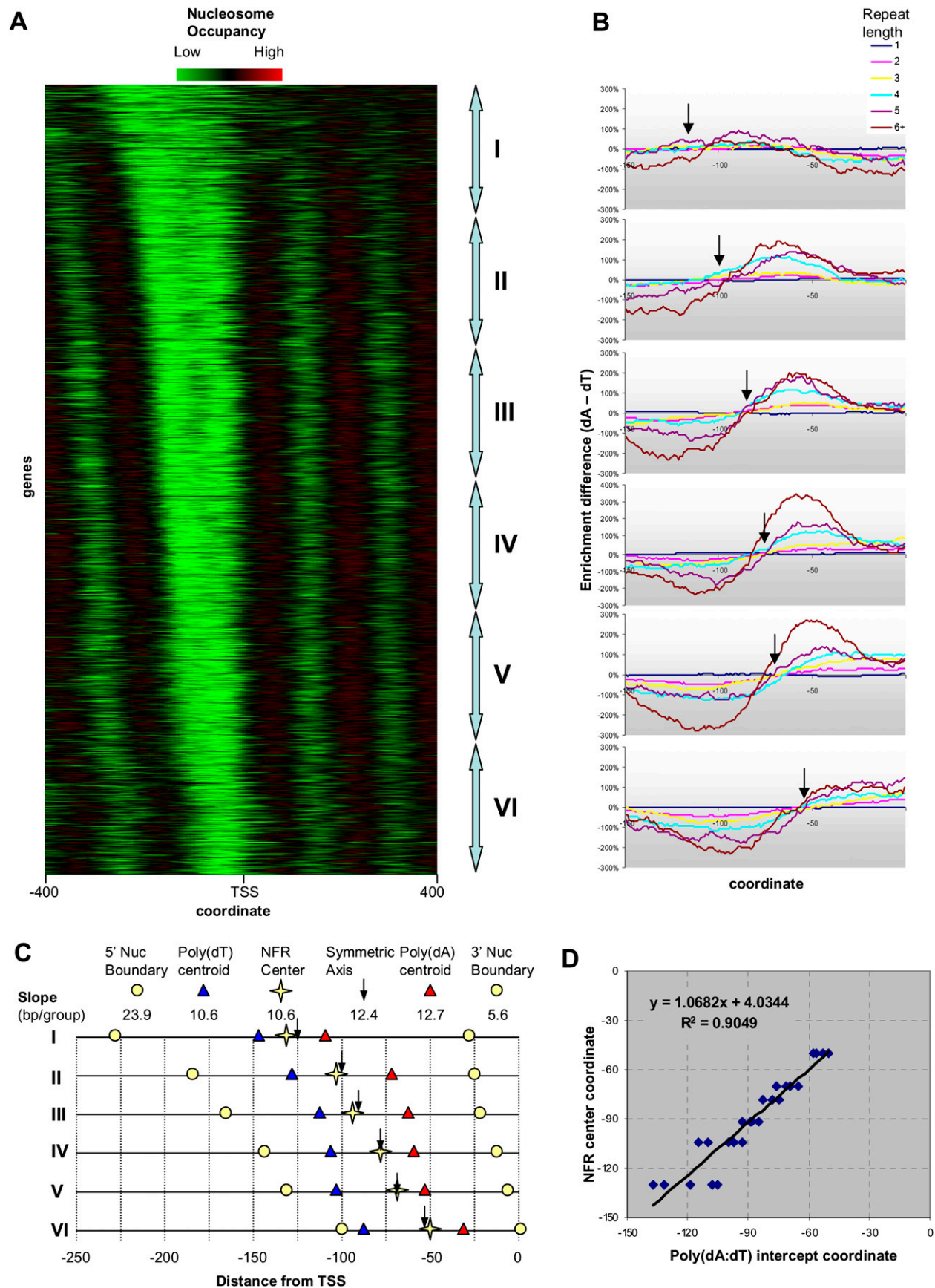
Figure 3. Poly(dA:dT) tracts track fine variations in NFR positions. (A) The class I promoters, which show a progressive narrowing of the NFR, are divided into six equal subgroups, I–VI. (B) Poly(dA:dT) tract enrichment differences for each subgroup. Arrows denote locations of symmetric axes for individual subgroups. (C) Schematic summary of the locations of six promoter elements in each promoter subgroup and represent the average number of base pairs an element shifts per subgroup of promoters. (D) Plot of NFR center coordinates versus poly(dA:dT) intercept coordinates. Multiple points for each subgroup represent intercepts for different tract length.
