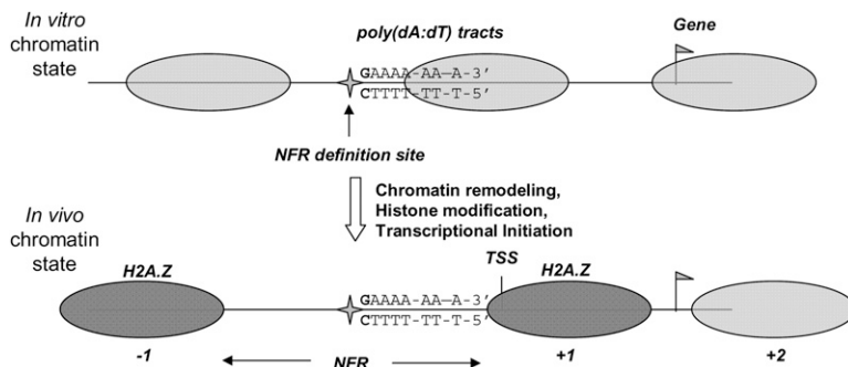
Figure 8. A model of how poly(dA:dT) tracts mediate extrinsic nucleosome-positioning effects. Illustrating a hypothetical role of poly(dA:dT) tracts in facilitating a the formation of an in vivo NFR during nucleosome assembly or remodeling. 5' G:C-capped poly(dA:dT) tracts, in conjunction with downstream uncapped tracts, may guide the activity of a chromatin-remodeling complex or transcription factor. The 5' capping residue may signal the initiation or termination of remodeling activity. This process may be coupled to the deposition of histone H2A.Z deposition into boundary nucleosomes. The NFR, once established, serves as the basis for subsequent transcriptional initiation events.
