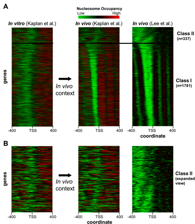
Figure 1. Comparison of in vitro and in vivo nucleosome maps at yeast promoters. (A) Nucleosome maps from tiling array data (Lee et al. 2007) for 2118 S. cerevisiae promoters were clustered using a self-organizing map (SOM) and visually partitioned into two groups (class I and class II). In vivo and in vitro nucleosome maps (Kaplan et al. 2008) were ordered according to the SOM. Maps were aligned according to transcriptional start sites determined using tiling arrays (David et al. 2006). (B) Close-up of the class II promoter class.
