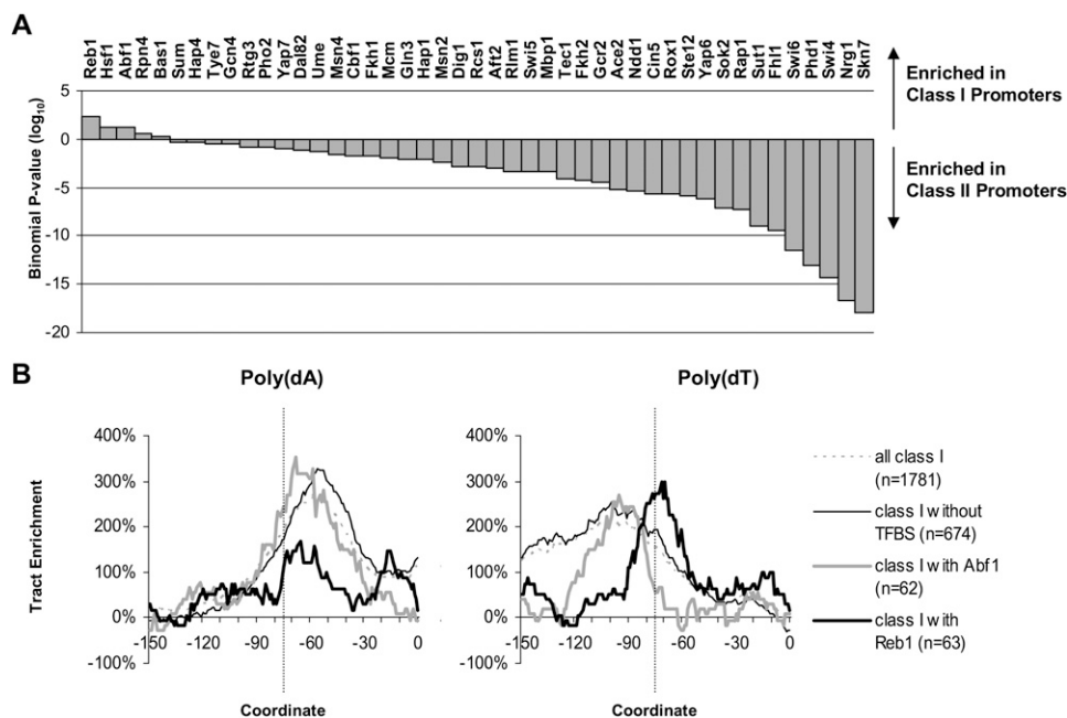
Figure 7. Poly(dA:dT) enrichments occur independently of transcription factor binding sites. (A) Ranking of transcription factors by overrepresentation of bound and functionally conserved sites in class I promoters based on annotated sites from MacIsaac et al. (2006). P-values were computed by modeling the distribution of TFBS between class I and class II promoters using a binomial distribution. The vertical axis gives the logarithm of the cumulative binomial probability of having the observed number of TFBS in a given class. Overrepresentation in class I promoters is shown by positive values and in class II promoters by negative values. (B) Poly(dA:dT) tract enrichments (length \geq 4 ) for class I promoters and subsets thereof: Abf1-containing promoters, Reb1-containing promoters, and TFBS-depleted promoters. TFBS-depleted promoters were selected by excluding promoters containing moderately bound ( P < 0.005 ) binding sites (no conservation requirement) for any of 118 TFs.
