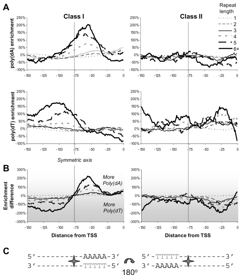
Figure 2. Poly(dA:dT) tract enrichment patterns in yeast promoters. (A) Poly(dA:dT) tract frequencies in class I and class II promoters are represented as relative percent enrichments over background tract frequencies. Tracts in the two orientations are considered separately and referenced as either poly(dA) or poly(dT) according to the downstream direction of transcription. Data are smoothed over 21-bp windows. Tracts of lengths 6 and greater were considered collectively for statistical accuracy. Coordinates are relative to transcription start sites (TSS). (B) Enrichment differences between poly(dA) and poly(dT) tracts as a function of promoter position; values above the x -axis indicate greater poly(dA) enrichment. The symmetric axis near -75 is indicated with a dashed line. (C) Illustrating the 180^\circ rotational (i.e., C_2 ) symmetry of poly(dA:dT) tracts with respect to the symmetric axis.
