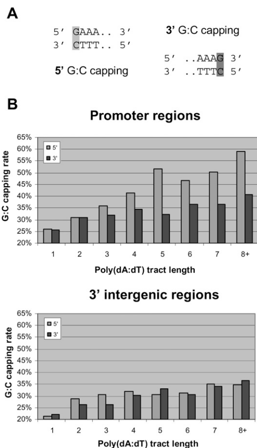
Figure 4. G:C capping of poly(dA:dT) tracts. (A) Illustrating the concept of poly(dA:dT) G:C capping. The poly(dA) strand preferentially terminates with G residues at both ends, while the poly(dT) strand preferentially terminates with C. The capping terminal is designated relative to the poly(dA) strand: GA_n and T_nC tracts, 5' capping; A_nG and CT_n , 3' capping. (B) G:C-capping rates at 5' and 3' termini over different tract lengths in promoter intergenic regions (from TSS to -150 ) and 3' intergenic regions (nonoverlapping with promoter sequences).
