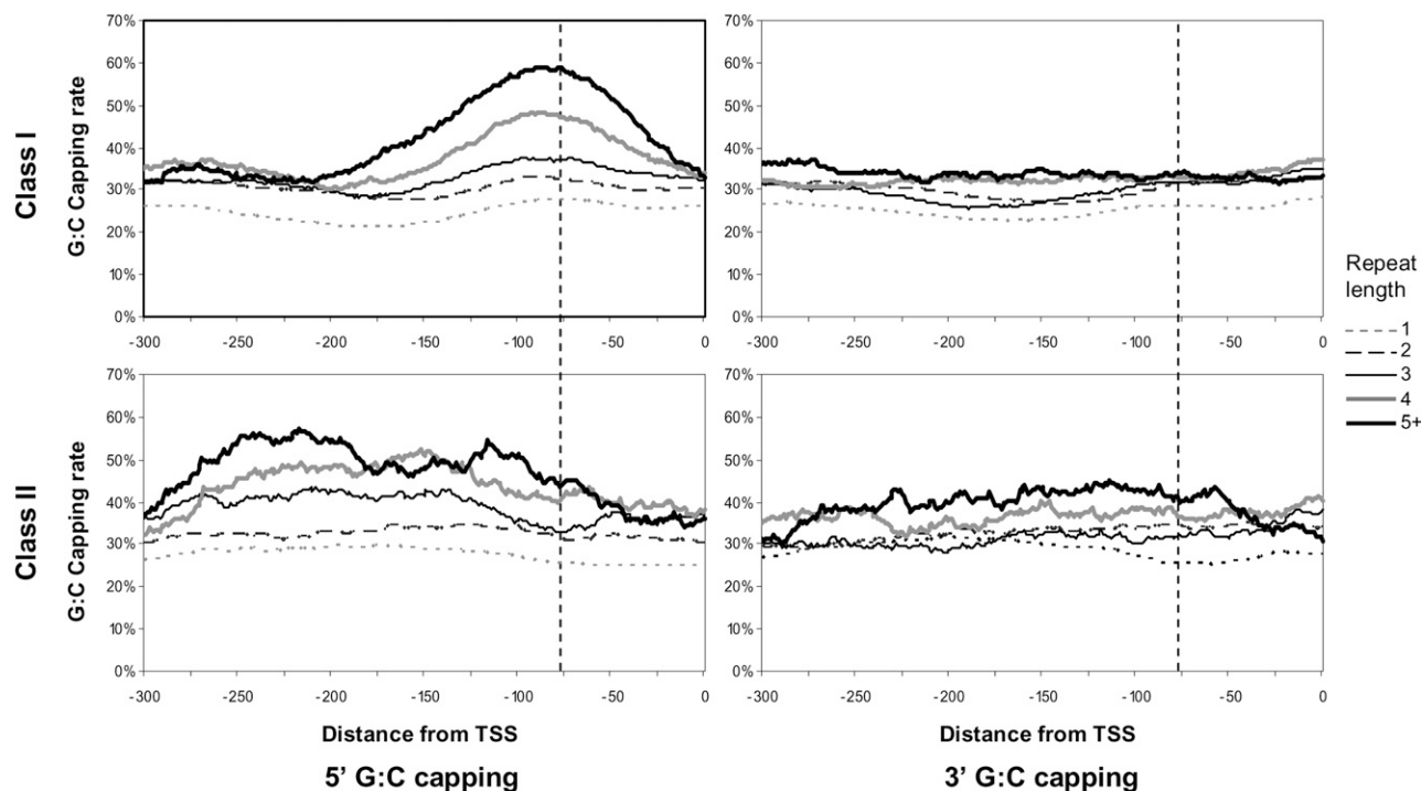
Figure 5. 5' and 3' G:C-capping rates, as functions from the TSS in class I and class II promoters. Patterns denote different poly(dA:dT) tract lengths; tracts 5 and longer were pooled for statistical accuracy. Vertical dashed line indicates the position of the symmetric axis for the average class I promoter.
