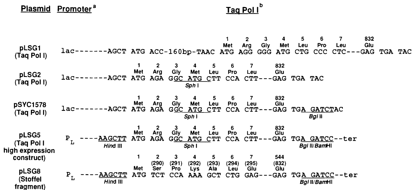
FIGURE 1 Taq Pol I expression constructions. Plasmids are described in the text. a Promoter-ribosome binding sites are: lac , \beta -galactosidase; P L , \lambda P L promoter/gene N ribosome binding site. b Taq Pol I codons are numbered above each sequence to show the amino-terminal codons and carboxy-terminal codons and how they were altered in the mutagenesis and recloning described in the text. Restriction endonuclease cleavage sites are underlined and labeled. The B. thuringiensis \delta -toxin retroregulator is indicated by ter. Numbers appearing in parentheses in pLSG8 refer to the corresponding codon numbering of the full-length gene.
