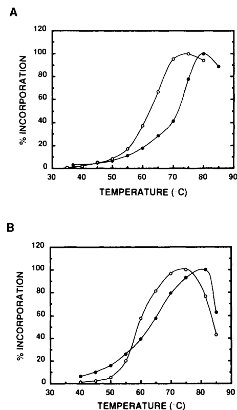
FIGURE 6 Thermal activity profiles of purified recombinant Taq DNA polymerases. Activity is represented as percent of maximum dCMP incorporation for each template and enzyme (assays performed under previously determined optimum conditions). (A) Taq Pol I with: (●) activated template (100% represents 114 pmoles of dCMP incorporated); (○) M13 primer-template (100% represents 80 pmoles of dCMP incorporated). (B) Stoffel fragment with: (●) activated template (100% represents 150 pmoles of dCMP incorporated); (○) M13 primer-template (100% represents 130 pmoles of dCMP incorporated).
