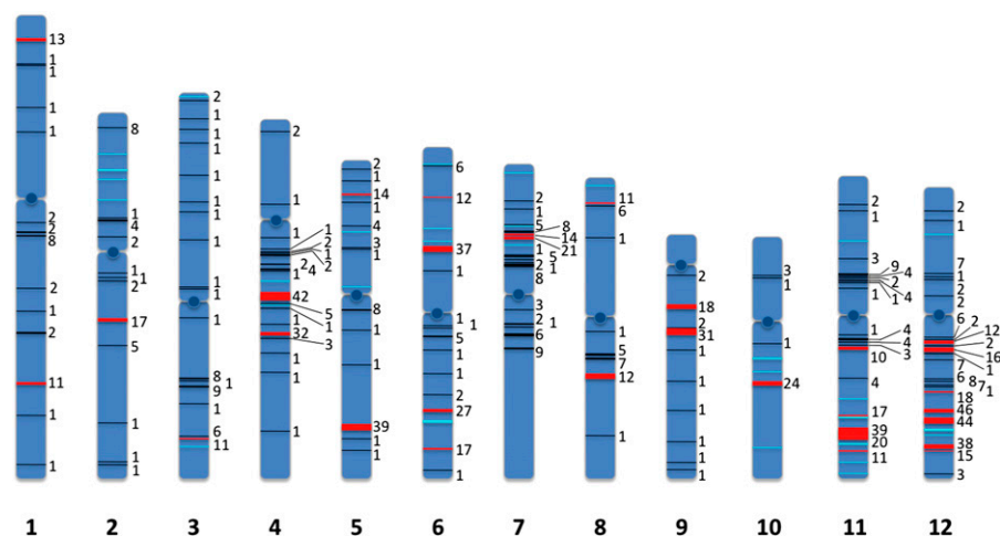
Figure 1. Distribution of 21-mer superclusters and phased 24-mer clusters in the rice genome. Regions of 21-mer clusters are represented as black lines ( <10 clusters) or if they are superclusters as red lines ( \geq 10 clusters). Phased 24-mer clusters are represented as cyan lines. The number of individual clusters within a region is indicated next to the line.
