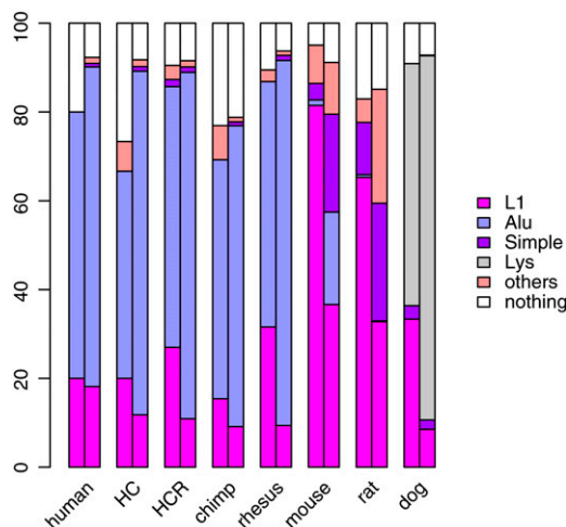
Figure 7. Overrepresentation of alignable pairs of L1 repeats in the breakpoints of mammalian reversals. In each lineage, the first bar represents the proportion of reversals for which the best BLAST alignment overlaps a particular repeat family, and the second bar represents the proportion of reversals that is expected to overlap a particular repeat family based on size-matched random simulations. This analysis is restricted to the 550 reversals with breakpoints defined within 100 kb.
