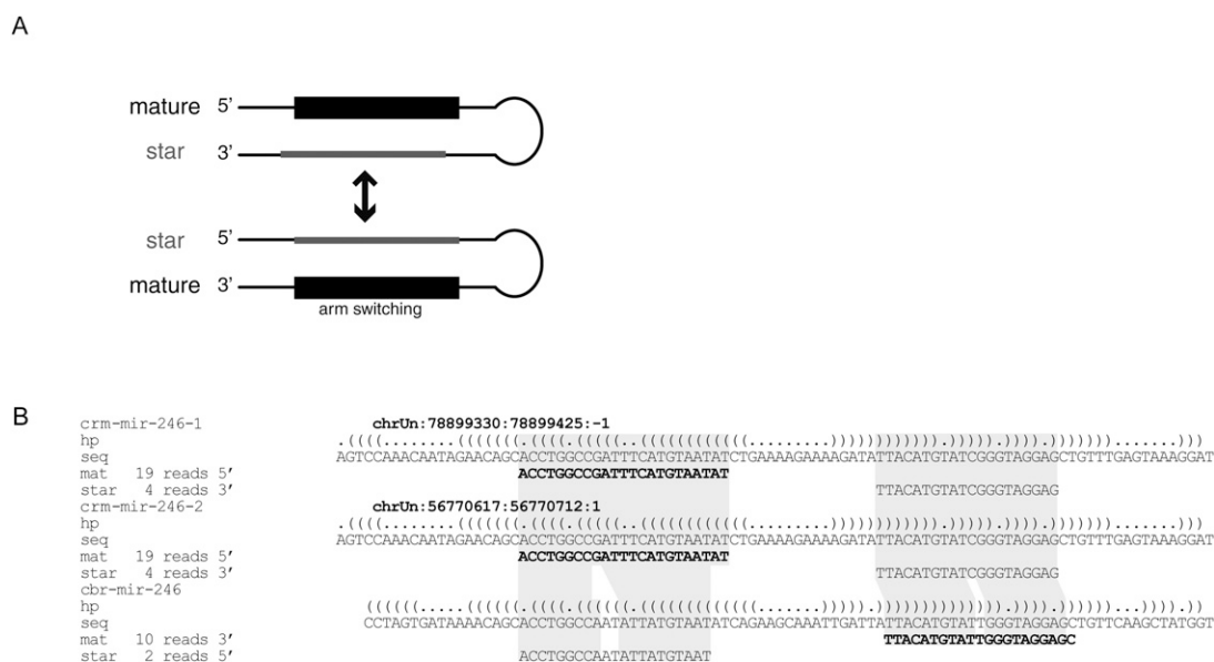
Figure 3. Arm-switching model of miRNA evolution. (A) Schematic representation of arm switching. In one miRNA hairpin, the 3' arm provides the mature miRNA. In a slightly modified hairpin, the mature miRNA is the one that comes from the 5' arm. (B) An example of arm switching. According to our cloning data, the duplicated loci of mir-246 in C. remanei express the 5' arm as mature miRNAs, whereas this locus in C. briggsae expresses the 3' arm as mature miRNA.
