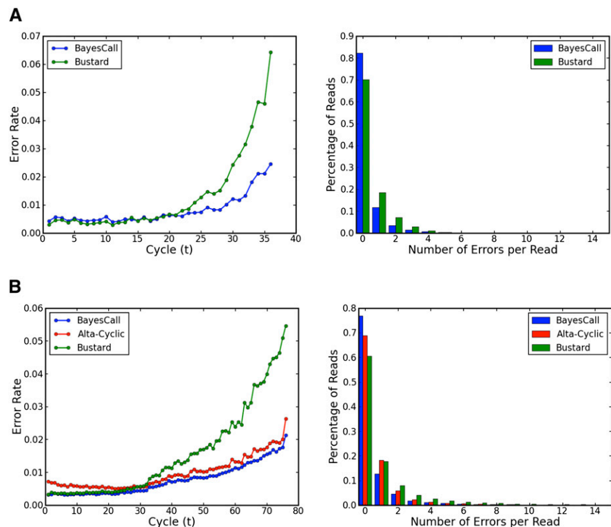
Figure 6. Average per-cycle error rates and histograms for the number of errors per read. BayesCall had substantially lower error rates in later cycles compared with Bustard, and the difference tended to increase with cycles. Further, BayesCall produced substantially more perfect reads than did Bustard. Alta-Cyclic was run only on the 76-cycle phiX174 data set. BayesCall had a lower average error rate than that of Alta-Cyclic’s for all cycles. Note that although Alta-Cyclic is more accurate than Bustard in later cycles, the opposite is true for earlier cycles. (A) Results for the 36-cycle data set. (B) Results for the 76-cycle data set.
