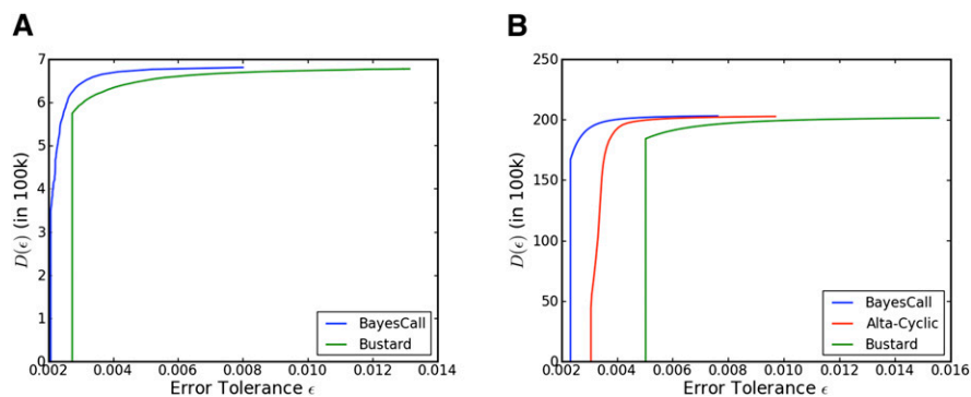
Figure 8. Discrimination ability D(\epsilon) of quality scores at error tolerance \epsilon . We define D(\epsilon) as the number of correctly called bases at error tolerance \epsilon . BayesCall maintains a high discrimination ability which outperforms both Bustard's and Alta-Cyclic's. (A) Results for the 36-cycle phiX174 data set. (B) Results for the 76-cycle phiX174 data set.
