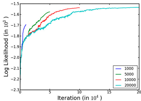
Figure 2. Convergence of simulated annealing with 1000, 5000, 10,000, and 20,000 total iterations. The temperature parameter in the i th iteration of simulated annealing is taken as (n - i + 1)/n , with n being the total number of iterations. Although using a larger value of n maximizes the likelihood slightly better, the inferred MAP estimate of \mathbf{S}_k does not change so much.
