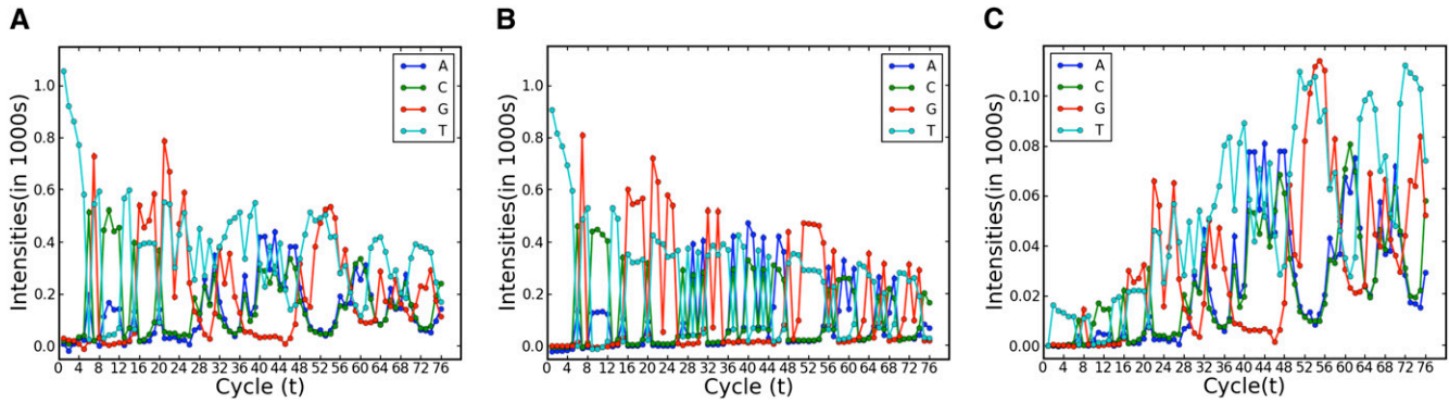
Figure 4. Observed intensities and the decomposition of \mu_{t,k} for a particular cluster k in the 76-cycle phiX174 data. (A) Observed intensities I_{t,k} . (B) The contribution of \Lambda_{t,k} X_{t,k} S_k Q_t^\omega to \mu_{t,k} . (C) The contribution of the residual effect \alpha_t(1-d) I_{t-1,k} .
