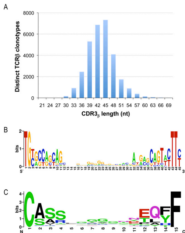
Figure 5. CDR3 \beta nucleotide length distribution and sequence composition of the most abundant CDR3 \beta length. To explore CDR3 \beta length variation we used a precise length criterion, defined as all bases between the last cysteine of TRBV and the phenylalanine in the TRBJ segment motif FGXG. Of the 33,664 total clonotypes, 30,366 could be classified in this manner, and the length distribution of this subset was plotted (A). The most frequently observed length was 45 nt. For the subset of clonotypes with 45 nt CDR3 \beta sequences, we created logos for the nucleotide (B) and inferred amino acid (C) composition, using WebLogo (Crooks et al. 2004).
