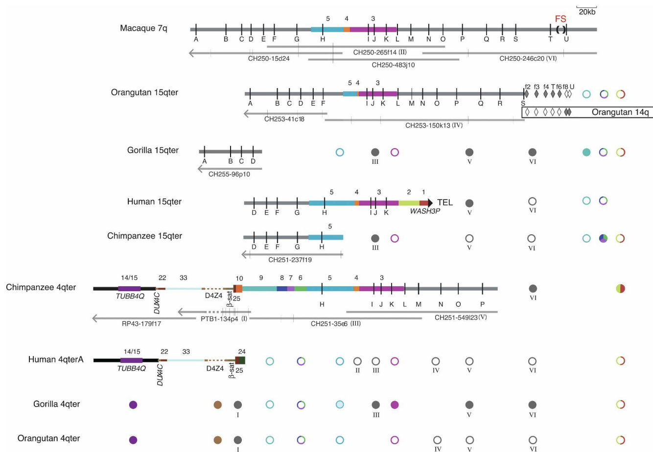
Figure 2. Sequence content of the fission site region of macaque chromosome 7 and chromosomes 15q and 4q subtelomeres in primates, as compiled from sequenced BACs and targeted FISH and PCR assays. The annotated thick horizontal lines indicate sequence contigs derived from non-human BACs or the human genome assembly. The large filled triangle at the right end of human 15q indicates it as the only one of these sequence contigs to reach the terminal telomere-repeat arrays. Vertical black lines represent OR genes identified by letters A–U (see Supplemental Table 6 for official nomenclature for these genes). The fission site (FS), indicated by ( ), lies between ORs T and U. Colored bars represent sequence blocks known to be subtelomerically duplicated in the human genome (Linardopoulou et al. 2005); blocks 5, 4, and 3 derive from the fission site region. Horizontal gray lines indicate additional sequences orthologous to the rhesus macaque fission-site region. Orange-brown and gray dashes indicate unsequenced D4Z4 arrays in contigs and BAC PTB1-134p4, respectively. Filled or open diamonds indicate PCR assays on flow-sorted orangutan chromosomes 15 or 14 that were positive or negative, respectively (Supplemental Table 3). The spans of the constituent sequenced BACs are indicated by the thin gray lines under each non-human contig; vertical gray lines on these tracks indicate gaps in sequence contigs; left-pointing arrowheads indicate that the BAC sequence extends toward the centromere from portion shown. BACs used for FISH are indicated by roman numerals I–VI in parentheses. Circles summarize the results of FISH assays for sequence whose presence is not already evident from the sequence contigs; filled or open circles indicate the presence or absence, respectively, of a cumulative signal-intensity score at the cytogenetic location exceeding 25% of the maximum cumulative score observed in the experiment (Trask et al. 1998 for block 3; Supplemental Table 2). Note that the presence of a FISH signal does not necessarily mean that the entire probe sequence resides at that location. Gray circles labeled with roman numerals I–VI represent FISH results with BACs constituting the contigs. Colored circles correspond to block-specific FISH probes; multicolored circles indicate that the FISH probe spanned more than one block. Circles for gorilla 4q represent a compilation of FISH results (Supplemental Table 2) and our PCR assays for blocks 9, 8, 7, 6, and 5 sequences in 4q-derived, D4Z4-containing gorilla BACs identified by Bodega et al. (2007) (Supplemental Table 3). The block-5 circle is partially shaded to indicate that gorilla 4q is FISH negative for this sequence, but these gorilla 4q BACs are PCR positive only for the most distal block 5 assays. Note that FISH assays detect the presence/absence, but not the order, of sequences in a given subtelomere. Wherever possible, FISH-result symbols are aligned with the corresponding probe's sequence in at least one contig; the FISH symbols for blocks 1/2, 9, and 6/7/8 are shown at the far right to indicate that these probe sequences, when detected by FISH, most likely lie telomeric of the sequence in the contigs. The sequence contigs are drawn to scale and aligned to facilitate comparison of their contents: macaque 7q, orangutan 15q, and human 15q contigs are aligned at OR gene I; chimpanzee 15q and 4q are aligned to human 15q at gene H; gorilla 15q is aligned to human 15q at gene D; human 4q is aligned to chimpanzee 4q at TUBB4Q . The diagrams of sequence contigs are truncated at arrowheads just proximal of gene A to exclude a complex region of tandem repeats that proved difficult to align across species, and the diagram for PTB1-134p4, is truncated at an arrowhead to indicate the extent of curated sequence from this BAC.
