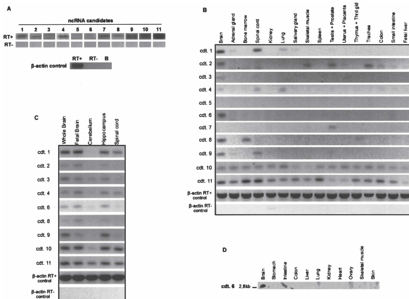
Figure 4. Expression of predicted ncRNA candidates by RT-PCR and Northern blot analysis. (A) Strand-specific RT-PCR analysis of ncRNA candidates on human RNA pools (see Methods). \beta -Actin was used as control, yielding PCR products in the presence of reverse transcriptase (RT+), but not in its absence (RT-). (B) Tissue-specific expression of ncRNA candidates as evaluated by RT-PCR analysis of human RNA samples. The same \beta -actin controls as for A were used. (C) Expression of ncRNA candidates within the human CNS as evaluated by RT-PCR analysis. The same \beta -actin controls as for A and B were used. (D) Expression of ncRNA candidate #6 as evaluated by Northern blotting of human RNA samples from 11 tissues.
