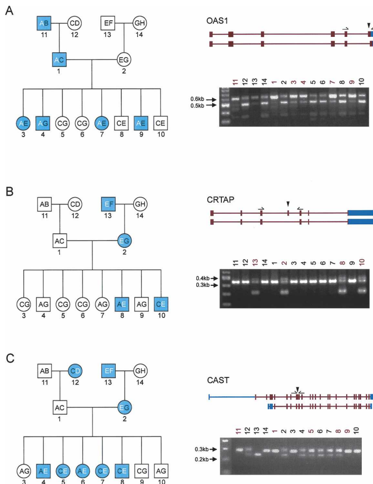
Figure 3. Heritability of alternative splicing. Inheritance of alternative splicing for genes (A) OAS1 , (B) CRTAP , and (C) CAST . Left panel shows pedigree structure of CEPH/UTAH family 1444 with the autosomal dominant inherited splice pattern as blue symbols. Haplotypes for each of the eight founder chromosomes are labeled A, B, C, D, E, F, G, and H, and the two inherited haplotypes of each family member are indicated within the symbol. The regulatory haplotype is shown as bold white text. Squares represent males, and circles represent females. CEPH/UTAH 1444 pedigree is labeled as follows: 1 (GM12739), 2 (GM12740), 3 (GM12741), 4 (GM12742), 5 (GM12743), 6 (GM12744), 7 (GM12745), 8 (GM12746), 9 (GM12847), 10 (GM12747), 11 (GM12748), 12 (GM12749), 13 (GM12750), and 14 (GM12751). The right panel shows the two transcript isoforms of the genes. Exon-body primers are shown above the flanking exons of the predicted alternatively spliced exons. Shown below the transcript isoforms are the RT-PCR results. Lanes are numbered from 1–14 according to the pedigree on the left.
