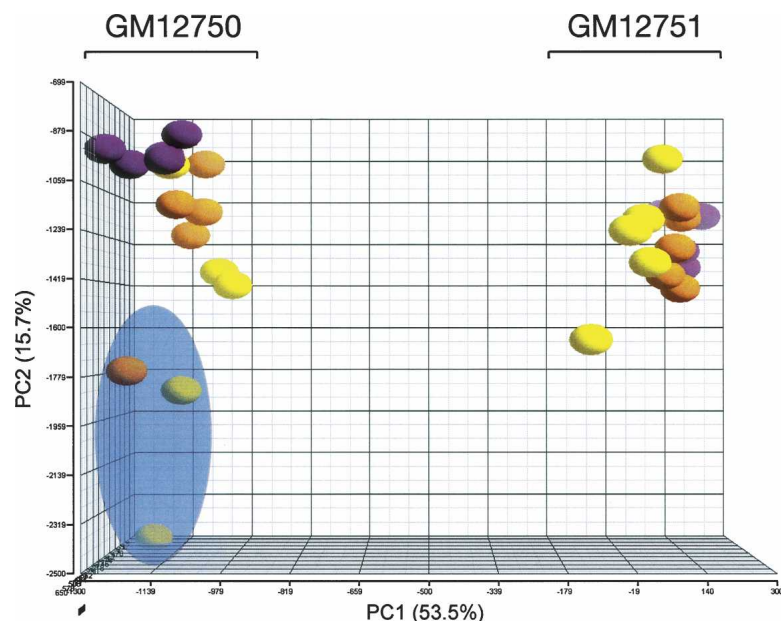
Figure 2. Principal component analysis. A three-dimensional plot of the splicing index data showing the three passages of five technical replicates each of individuals GM12750 and GM12751, on the left and right sides, respectively. The three biological replicates are shown as purple, orange, and yellow spheres, respectively. The three outliers that were removed from all subsequent analyses are shaded in a blue sphere. The percentage of variance attributed to principal components one and two is shown on the X- and Y-axes, respectively. Plots were created using the Partek Genomics Suite software package (Partek).
