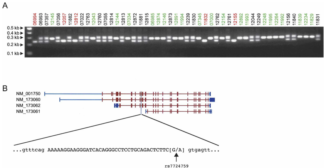
Figure 4. Association of alternative splicing and genotypes for the CAST gene. (A) RT-PCR of CAST exon against a panel of unrelated parents from each of the 30 HapMap CEU trios. Sample names are colored according to their genotype for SNP rs7724759 : homozygous GG (green), homozygous AA (red), and heterozygous AG (black). (B) Four known isoforms of the CAST gene are shown with their RefSeq accession numbers on the left and the candidate probe set shaded in gray. Shown below is the sequence of the exon in capital letters and flanked by the intronic sequence in lower case. The SNP rs7724759 is located at the last position of the exon and is a G to A substitution that disrupts the consensus splice site sequence.
