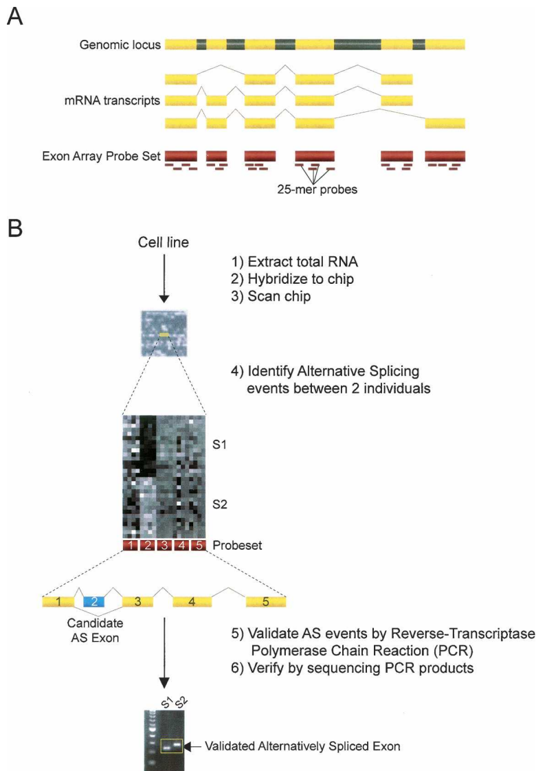
Figure 1. (A) Schematic for coverage of probe sets across the entire length of the transcript. Yellow regions are exons, whereas gray regions represent introns. The short dashes underneath the exon regions indicate individual probes of 25 nucleotides in length representing the probe set. The Affymetrix GeneChip Human Exon 1.0 ST Array allows for exon-level expression profiling in a single chip, and can interrogate over one million predicted exons within the human genome. (B) Flowchart for processing and analysis of chips to validation of alternative splicing events. Total RNA is extracted from the two cell lines ( n = 15 replicates per individual) and is transcribed to cDNA and labeled with biotin. The total cDNA is then hybridized to the exon chip, followed by washing and staining with an anti-streptavidin antibody. Chips are then scanned, and hybridization data are processed and analyzed by the Affymetrix Power Tools (version 1.6) software package. A splicing index is calculated for ~1.4 million probe sets covering one million exons. A subset of 20 alternative splicing events predicted between the two individuals using an unpaired t -test ( P < 8.915 \times 10^{-4} ) on the splicing index and other criteria (see Methods), are then validated by (1) RT-PCR using exon body primers flanking the probe set of interest and (2) sequencing of the RT-PCR products.
