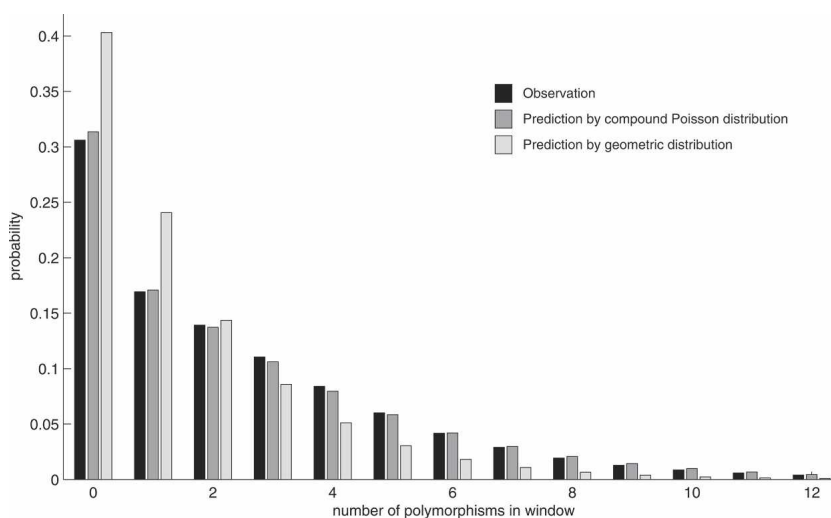
Figure 3. Probability distribution of polymorphism rates in 200-bp windows. Black bar indicates the probability that the given number of polymorphisms is observed in 200-bp windows. Dark gray bars indicate the probability predicted by the coalescent theory, which well fits our observation in the Ciona intestinalis genome. However, a geometric distribution, indicated by light gray bars, does not fit our observations.
