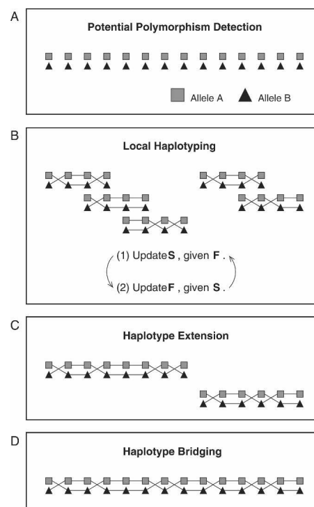
Figure 6. Overview of our haplotype reconstruction strategy. (A) In this step, Bayesian model selection is used to detect potential polymorphic sites along a genome. Two different alleles at each polymorphic site are represented by a triangle and a rectangle. In this figure, detected polymorphic sites run from the left-hand side to the right-hand side according to their genomic positions in an assembly. (B) We determine phases among detected polymorphisms by using a Gibbs sampling method. We focus on estimating reliable haplotypes from a small number of polymorphisms by repeating the following two steps: (1) update S based on F , (2) update F based on S . (C) If adjacent short haplotypes overlap and show a consistency, those haplotypes are combined. (D) Adjacent haplotypes are connected if the fragments spanning those adjacent haplotypes significantly support the connection.
