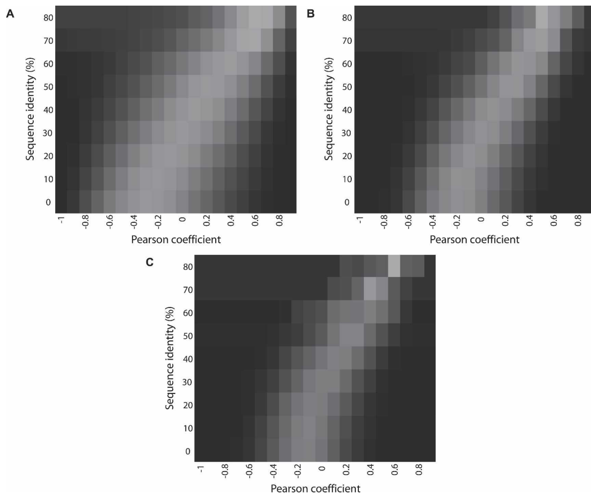
Figure 3. Cleavage/sequence correlation at various levels of sequence identity. Heat maps were created with Matrix2png (Pavlidis and Noble 2003), using the data from Supplemental Tables S5, S6, and S7 as input. (A) 10-mers; (B) 20-mers; (C) 30-mers. The intensity of each rectangle indicates the number of pairs of sequences in that cell, ranging from black (lowest) to white (highest).
