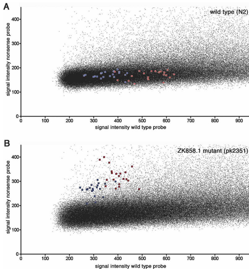
Figure 5. Array-based NIM analysis. The signal of the nonsense (vertical) versus the wild-type (horizontal) allele is plotted for wild-type worms (N2) (A) and pk2351 , containing an EMS-induced stopcodon in ZK858.1 (B). For nonmutated positions, the nonsense signal (vertical axis) is expected to be background, whereas the wild-type signal spreads over the X-axis, most likely reflecting GC content differences. A heterozygous mutation would have similar intensities for both the nonsense and wild-type allele, and these are thus expected to be located close to the diagonal in the figure. Microarrays with 390,000 features were used to assay part of the C. elegans genome-wide NIM collection. Every NIM was represented by four probes that were temperature-normalized ( T_m = 72^\circ\text{C} , probe length between 25 and 40 nt), representing the wild-type and mutant alleles for both DNA strands. The stop codon in ZK858.1 was represented 10 times (red, plus strand probes; blue, minus strand probes).
