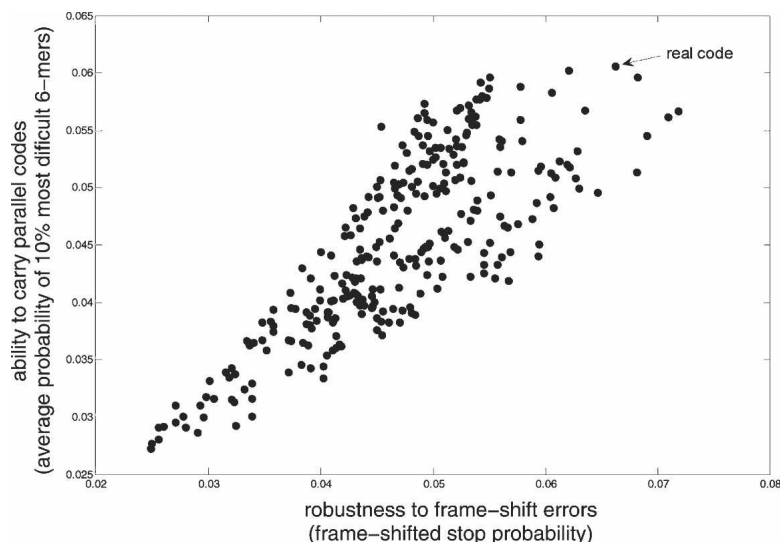
Figure 4. The parallel coding property is strongly tied to the translational frame-shift robustness property. Each point represents one of the alternative codes. The x -axis shows the probability of encountering a stop codon upon a frame-shifted event (average over +1 and -1 frame shift). The y -axis is the average probability of appearance of the 10% most difficult 6-mers. The arrow indicates the real code. The correlation between the two properties is 0.8. The real code is on the Pareto front, meaning that no alternative code is better than the real code in both properties. Similar results are obtained for n -mers of other sizes. Note that due to symmetries in the alternative codes with respect to the features studied (Supplemental material), multiple alternative codes often have the same values.
