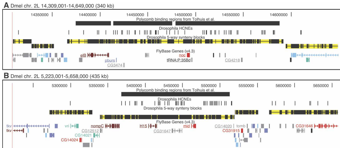
Figure 4. HCNE-clusters spanning coregulated genes and boundary agreement among syntenic blocks, HCNE clusters, and Polycomb binding regions. Gene models are colored by predicted core promoter type as in Fig. 2. Only selected genes are labeled. (A) The paralogous zinc finger genes elB and noc , implicated in tracheal and appendage development, have different, but partially overlapping, spatial expression patterns during embryonic development (Dorfman et al. 2002) and are coexpressed in larval leg and wing discs (Weihe et al. 2004). Among the five flies, elB and noc are in conserved microsynteny with a tRNA gene and at least three protein-coding genes (underlined), which have no evidence of being functionally related to elB or noc : pburs encodes a subunit of the hormone bursicon required for wing expansion and associated cuticle changes after flies emerge from pupae (Luo et al. 2005); CG3474 is predicted to encode a cuticle component; CG4218 is predicted to encode a protein of unknown function. (B) The paralogous T-box genes H15 and mid are involved in regulation of heart development and have similar spatial expression patterns during embryonic development (Miskolczi-McCallum et al. 2005; Reim et al. 2005). They are in conserved microsynteny with four other genes (underlined) among the five flies: CG12512 , predicted to encode a protein with an AMP-dependent synthetase and ligase domain; nompC , encoding a mechanosensory transduction channel (Walker et al. 2000); and two genes of unknown function. The developmental regulators vri (George and Terracol 1997) and tomb (Jiang et al. 2007) are centrally positioned in neighboring syntenic blocks. Two transcript isoforms are shown for tkv because it has two major transcription start sites with different types of core promoter predictions.
