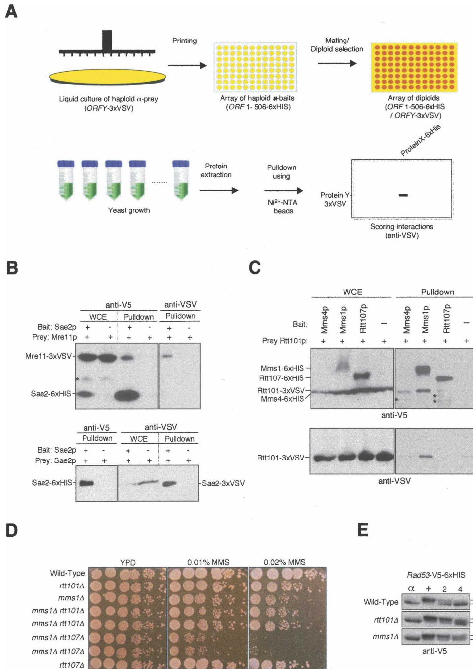
Figure 4. Using Cross-and-Capture to screen for novel PPIs. (A) Screening scheme. A strain containing a prey ( ORFY-3×VSV ) is combined with a set of different bait strains ( ORF1-506-6×HIS ) and diploids are selected. Extracts and Western blots are processed in parallel, and pull-downs of the prey protein are assessed. (B) Sae2p interacts with Mre11p and Sae2p . Pull-downs are from diploids expressing Mre11-3×VSV or Sae2-3×VSV as prey and Sae2-6×HIS as bait or no bait control (-). (C) Identification of the Rtt101p - Mms1p complex. Whole cell extracts (WCEs) and pull-downs probed with anti-V5 and anti-VSV antibodies are shown. Cells are treated with 0.02% MMS for 2 h before harvesting. Pull-downs are from diploids expressing Rtt101-3×VSV as prey and Mms1p , Mms4p , and Rtt107p as bait proteins (6×HIS) or no bait control (-). Nonspecific background signals in the Western blots are indicated (*). (D) Epistasis analysis for rtt101Δ and mms1Δ compared to rtt107Δ combined with mms1Δ . Cells are grown to mid-log phase and analyzed by spot assay in fivefold serial dilutions on YPD, YPD + 0.01% MMS, and YPD + 0.02% MMS. Pictures were taken after 2–3 d at 30°C. (E) Phosphorylation status of Rad53p (P) was determined by blotting Rad53-6×HIS from wild type, rtt101Δ , and mms1Δ strains with anti-V5 at indicated time points. Cells are arrested in G1 for 2 h with \alpha -factor ( \alpha ) and released into YPD containing 0.033% MMS for 2 h (+). Cells are then incubated with fresh YPD, and samples are collected after 2 and 4 h.
