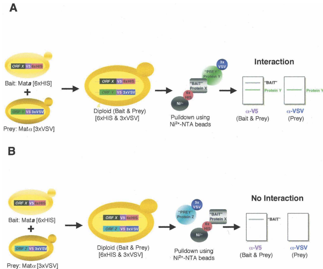
Figure 1. Cross-and-Capture Assay. (A,B) A strain containing the bait ORFX tagged with a V5 epitope and six histidines ( 6\times\text{HIS} ) is crossed with strains that contain prey ORFY or ORFZ tagged with a V5 epitope followed by a triple VSV tag ( 3\times\text{VSV} ). Diploids, which express both tagged bait and prey, are grown on selective medium. Protein extracts from the diploids are then incubated with nickel beads ( \text{Ni}^{2+} -NTA), allowing isolation of bait (Protein X- 6\times\text{HIS} ) and bait-associated prey protein (Protein Y- 3\times\text{VSV} ) (A), whereas a non-interacting protein (Protein Z- 3\times\text{VSV} ) will not bind (B). Proteins are then separated by SDS-PAGE, and blots are probed for bait and prey (anti-V5 antibody) and specifically for the prey (anti-VSV antibody) by immunoblot.
